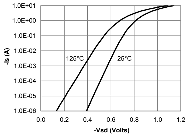
Figure 6: Body-Diode Characteristics
