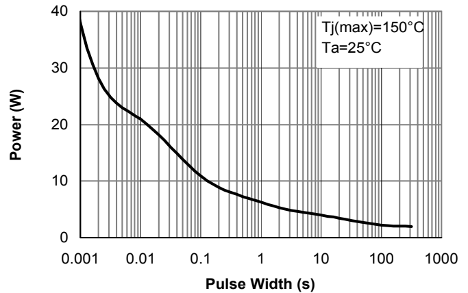
Figure 10: Single Pulse Power Rating Junction-to-Ambient (Note 5)
