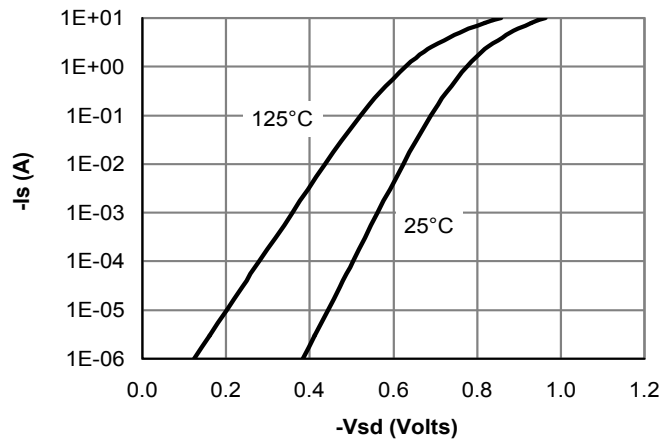
Figure 6: Body-Diode Characteristics
