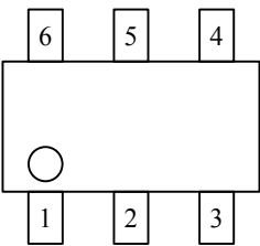
TSOP-6(TOP VIEW)
