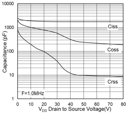
Fig.7 Capacitance
