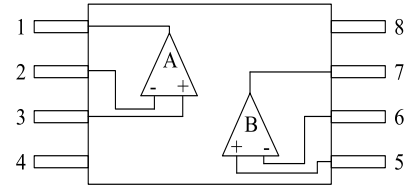
TSSOP-8(TOP VIEW)
