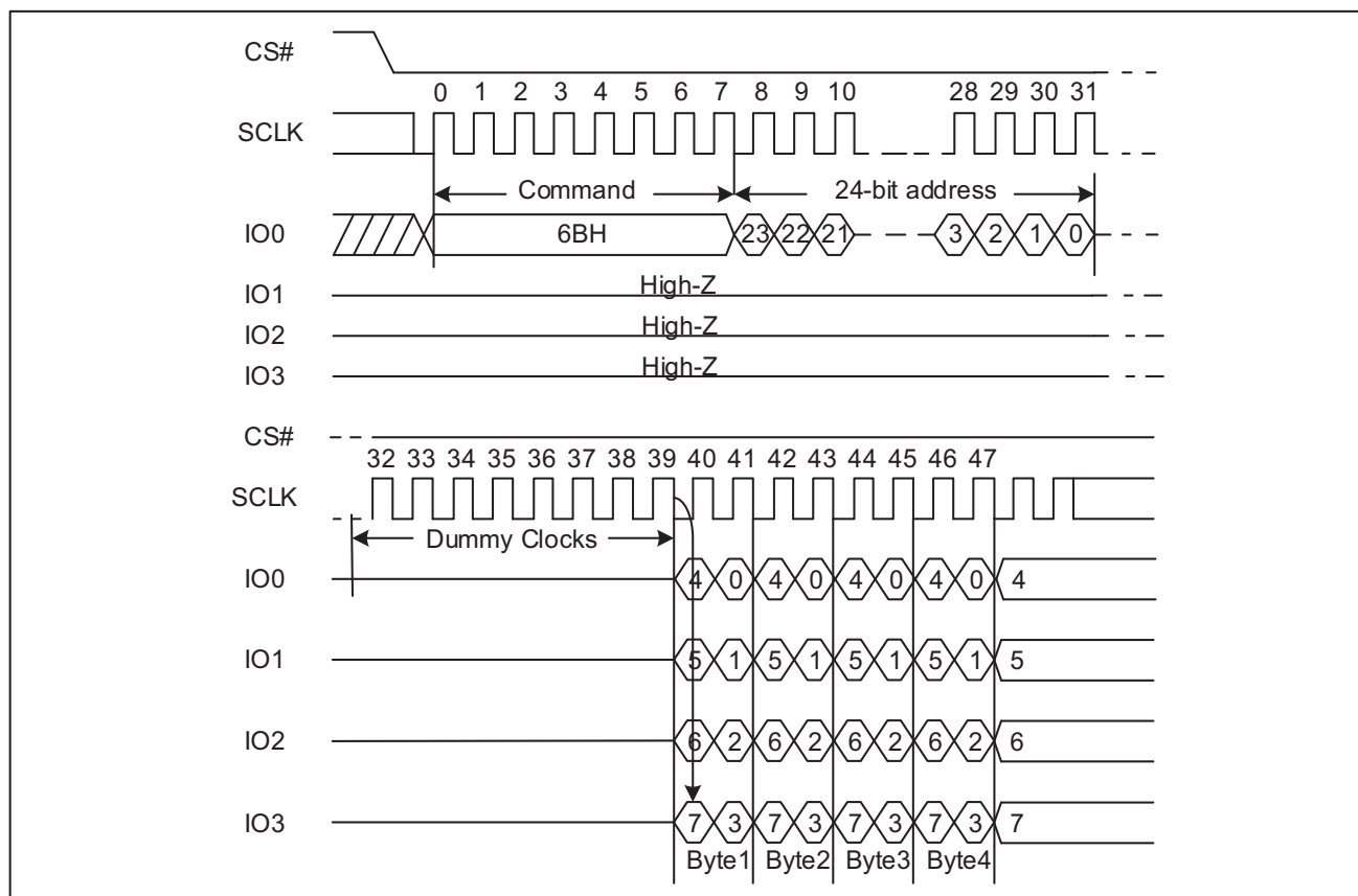
Figure 11. Quad Output Fast Read Sequence Diagram
