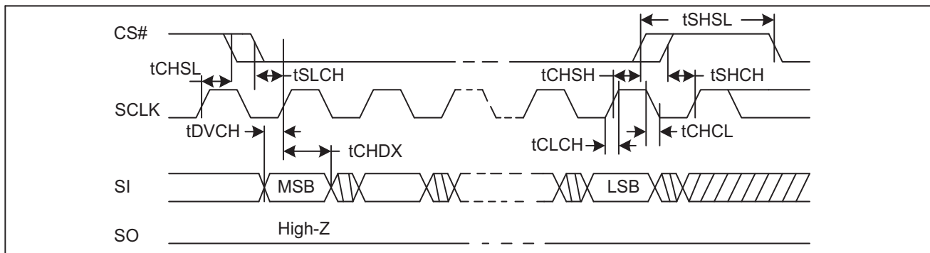
Figure 39. Input Timing
