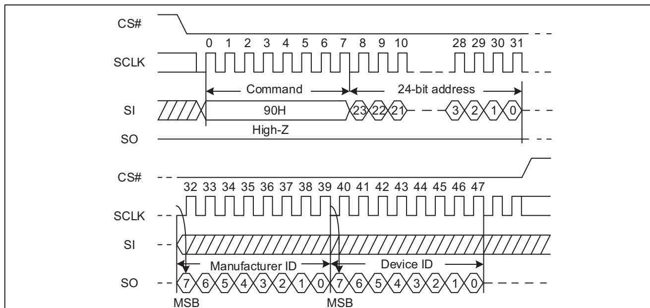
Figure 23. Read Manufacturer ID/ Device ID Sequence Diagram
