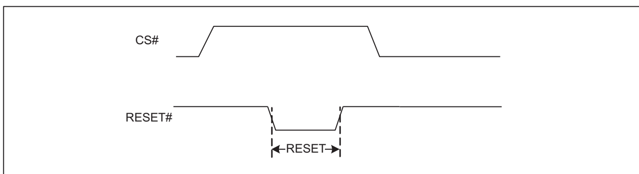
Figure 2 RESET Condition
