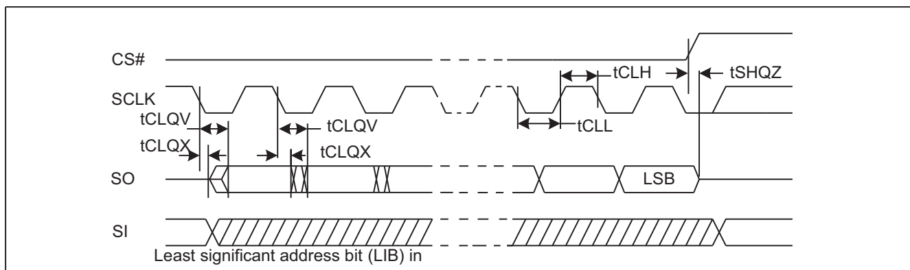
Figure 40. Output Timing
