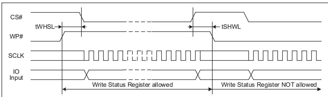
Figure 42. WP# Timing
