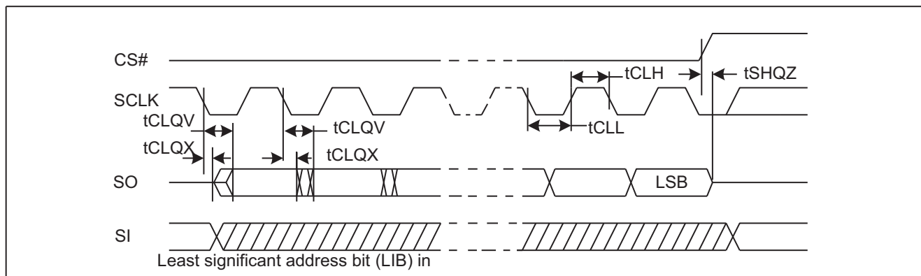
Figure 39. Output Timing
