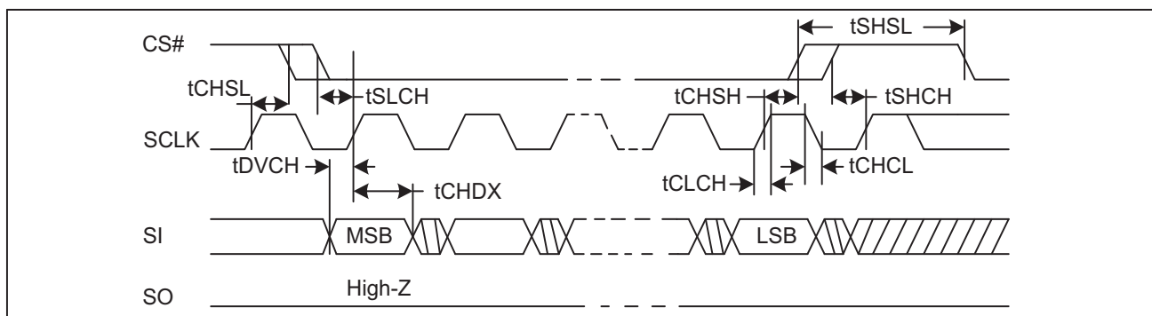
Figure 38. Input Timing
