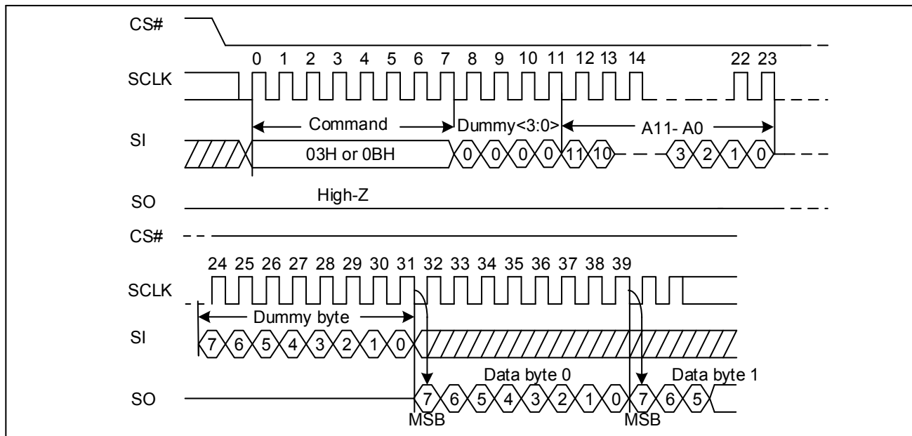
Figure 8-2. Read From Cache Sequence Diagram
