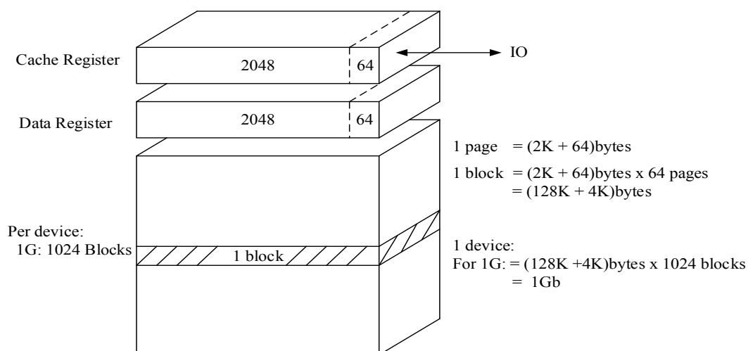
Figure 3. Array Organization
