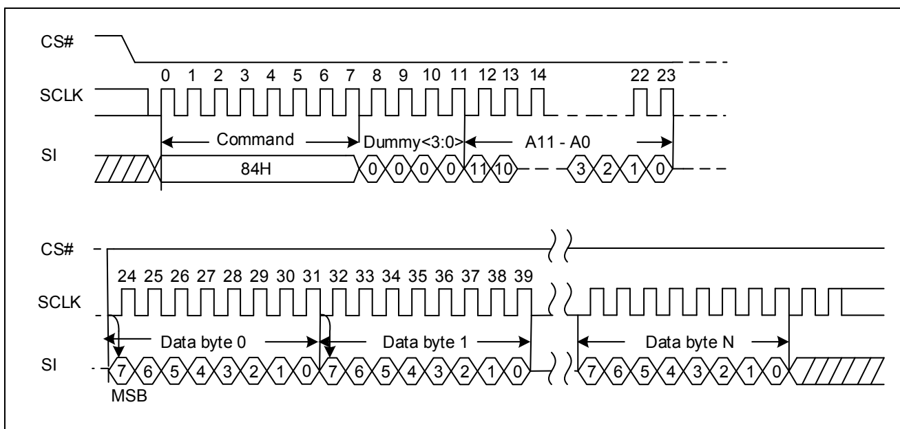
Figure 9-4. Program Load Random Data Sequence Diagram
