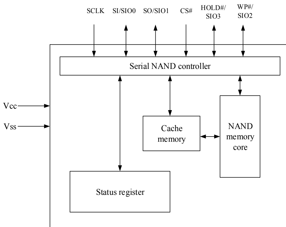
Figure 2-2. Block Diagram
