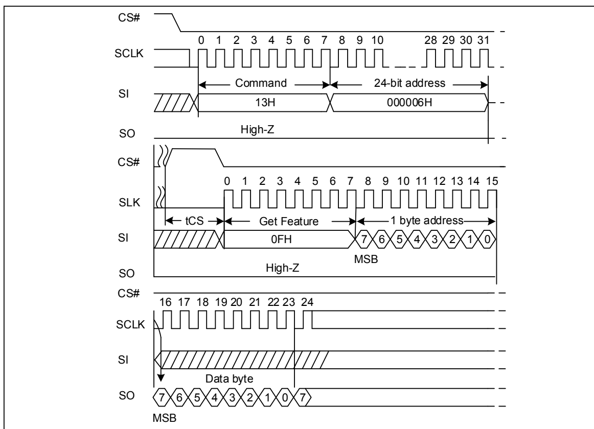
Figure 8-7. Read UID to cache and Get Feature command Sequence Diagram one
