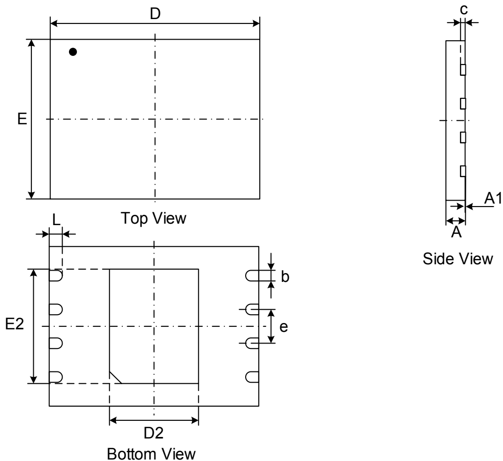
Figure 20-1. WSON8 (8*6mm)
