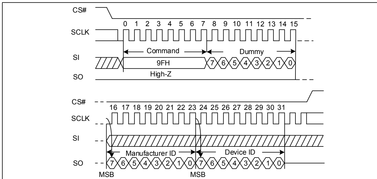
Figure 8-6. Read ID Sequence Diagram
