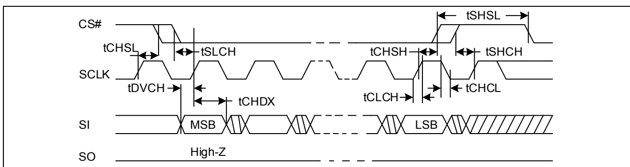
Figure 18-1. Serial Input Timing
