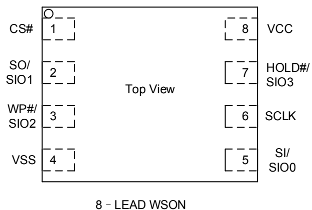
Figure 2-1. Connect Diagram
