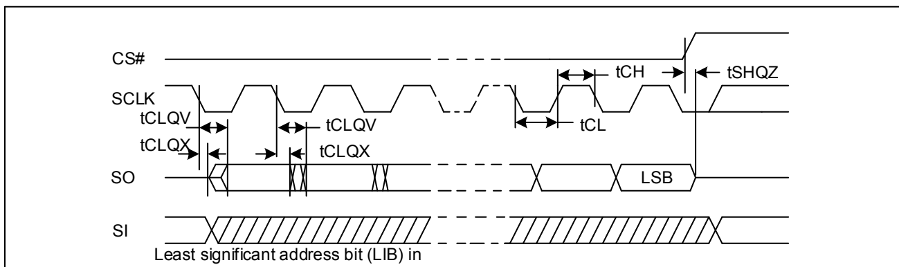
Figure 18-2. Output Timing
