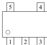
SOT-25(TOP VIEW)
