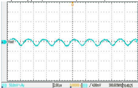
Output Rippie (12V \Rightarrow 3.3V, Load=0A)
