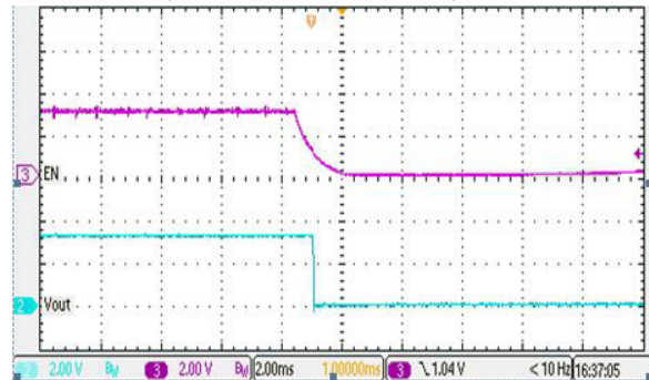
Shut Down (12V \Rightarrow 3.3V, Load=2A)
