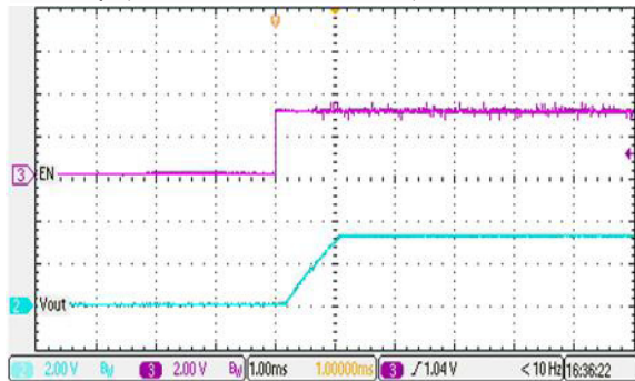
Start Up (12V \Rightarrow 3.3V, Load=2A)
