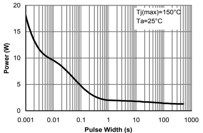
Figure 10: Single Pulse Power Rating Junction-to-Ambient (Note 5)
