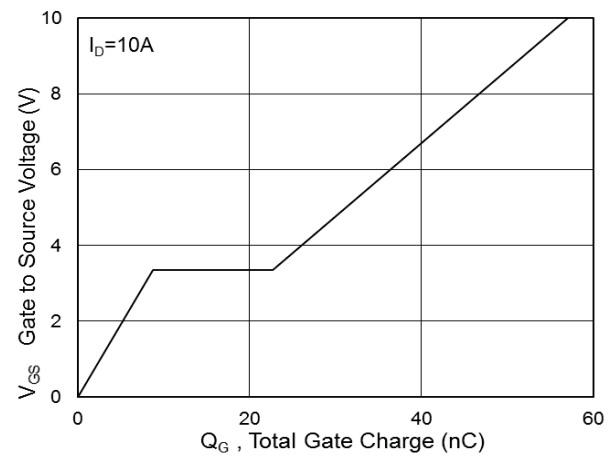
Fig.4 Gate-Charge Characteristics
