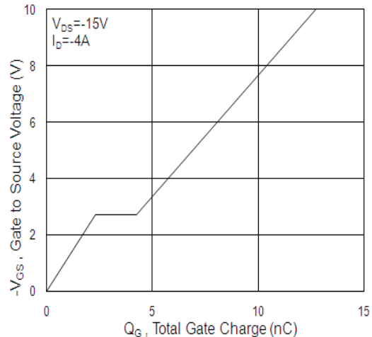
Fig.4 Gate-Charge Characteristics
