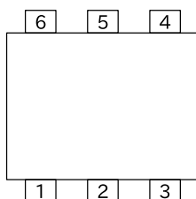
SOT-563(TOP VIEW)
