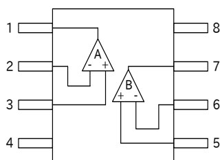
SOP-8(TOP VIEW)
