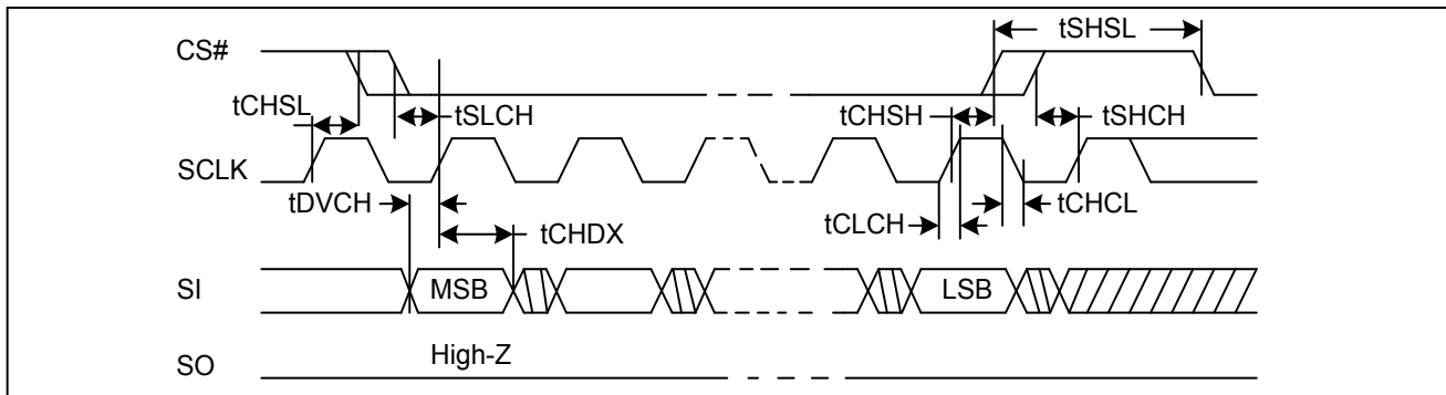
Figure 38. Input Timing
