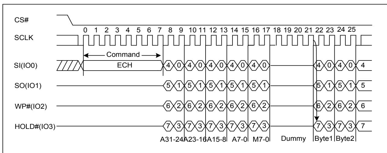
Figure 34. Quad I/O Fast Read with 4-Byte Address Sequence Diagram (M5-4 \neq (1, 0), ADS=0 or ADS=1)
