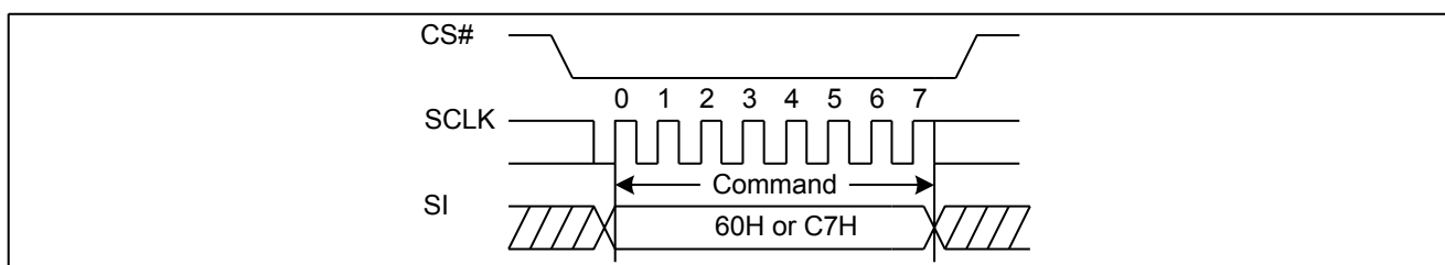
Figure 52. Chip Erase Sequence Diagram
