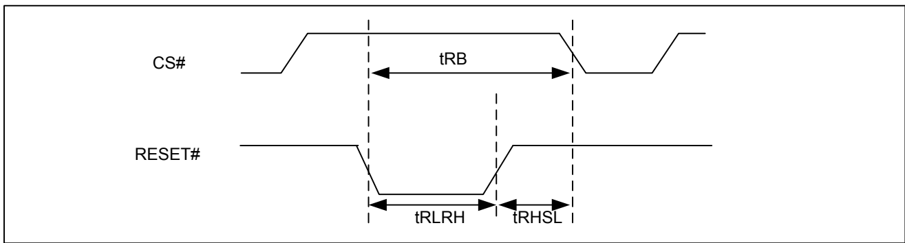
Figure82. RESET Timing
