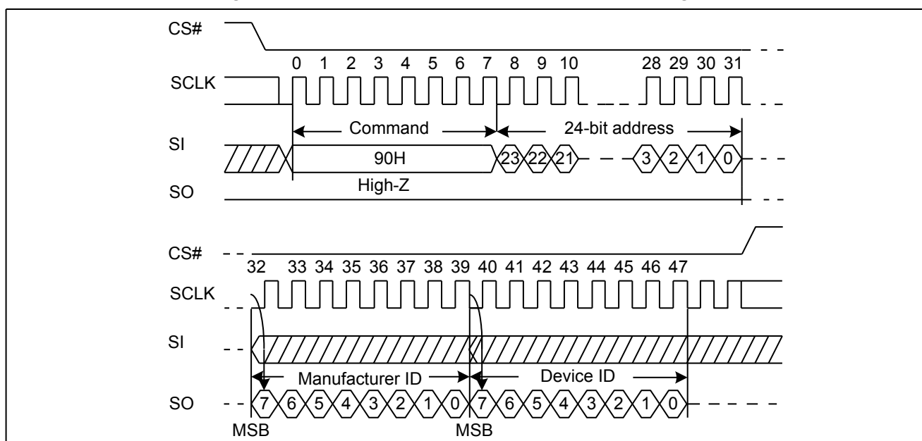
Figure 61. Read Manufacture ID/ Device ID Sequence Diagram
