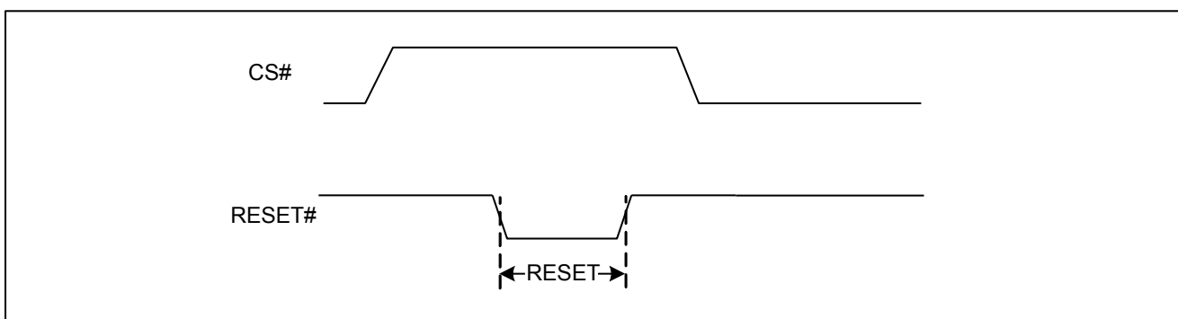
Figure 4 RESET Condition
