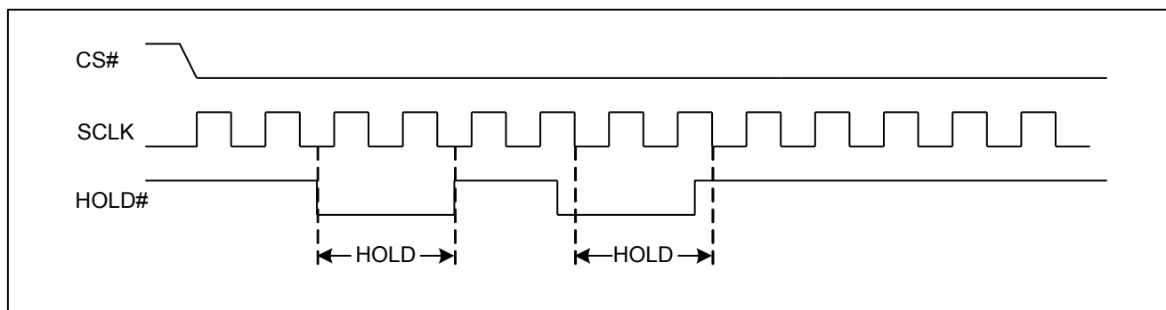
Figure 3 Hold Condition
