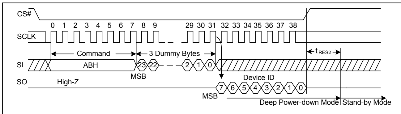
Figure 60. Release Power-Down/Read Device ID Sequence Diagram
