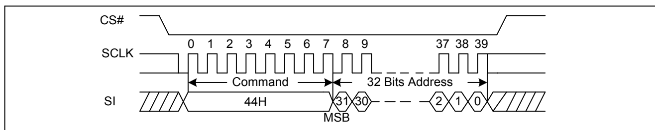
Figure68.Erase Security Registers command Sequence Diagram (ADS=1)
