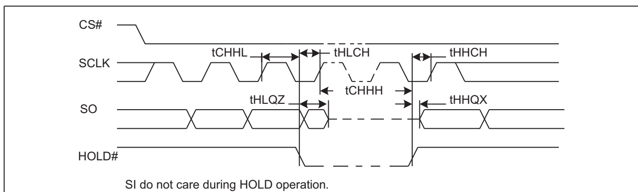
Figure 41. Hold Timing
