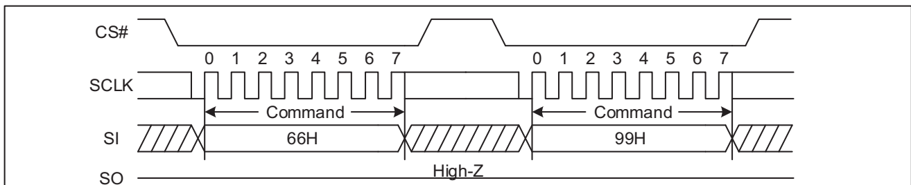
Figure 28. Enable Reset and Reset command Sequence Diagram
