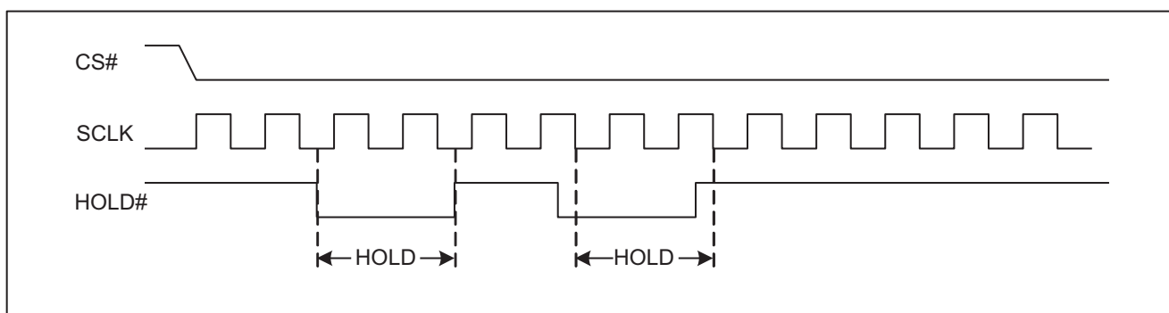
Figure 1 HOLD Condition
