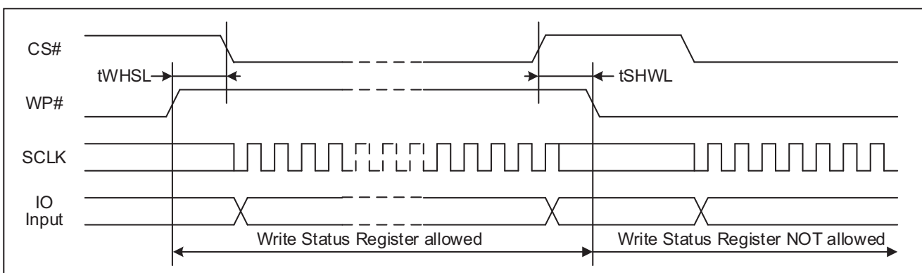
Figure 42. WP# Timing
