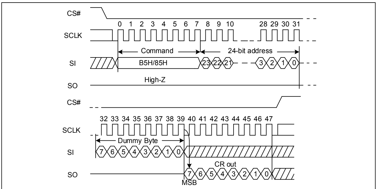
Figure 25 Read Configuration Registers Sequence Diagram (SPI)
