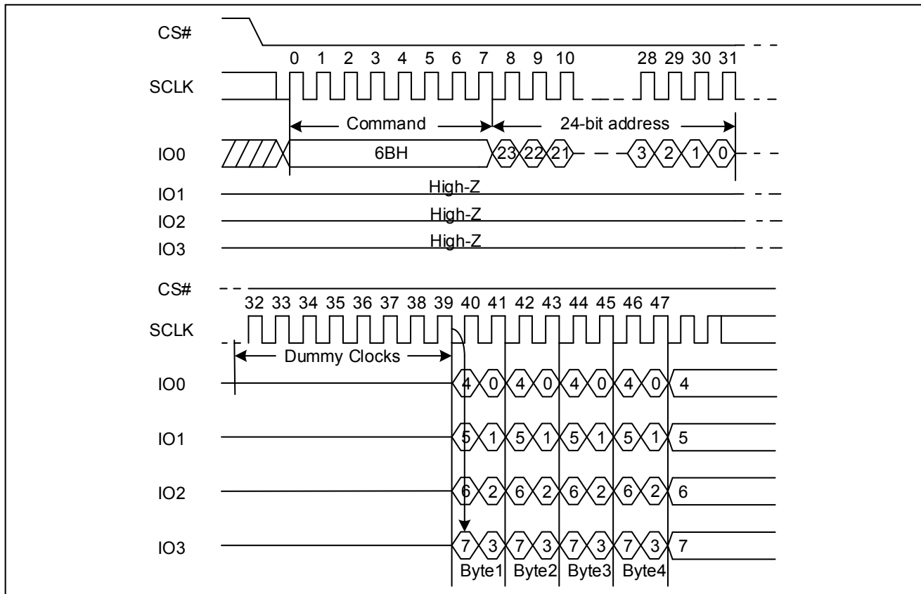
Figure 32 Quad Output Fast Read Sequence Diagram (SPI)
