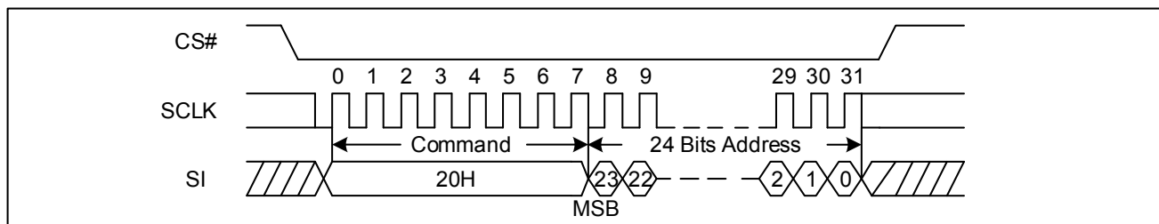
Figure 46 Sector Erase Sequence Diagram (SPI)
