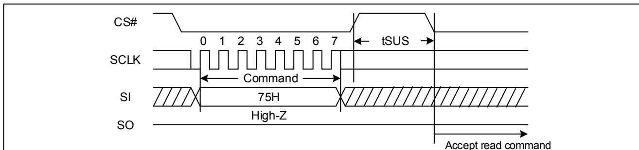
Figure 64 Program/Erase Suspend Sequence Diagram (SPI)
