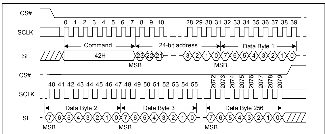
Figure 70 Program Security Registers command Sequence Diagram (SPI)
