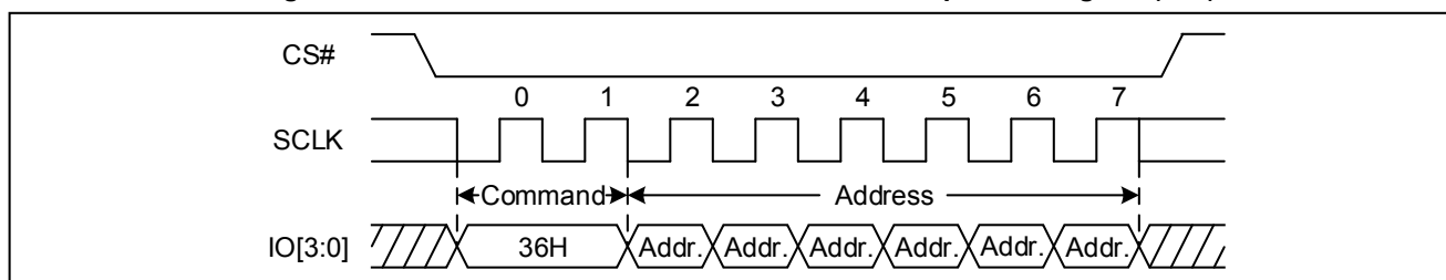
Figure 75 Individual Block/Sector Lock command Sequence Diagram (QPI)
