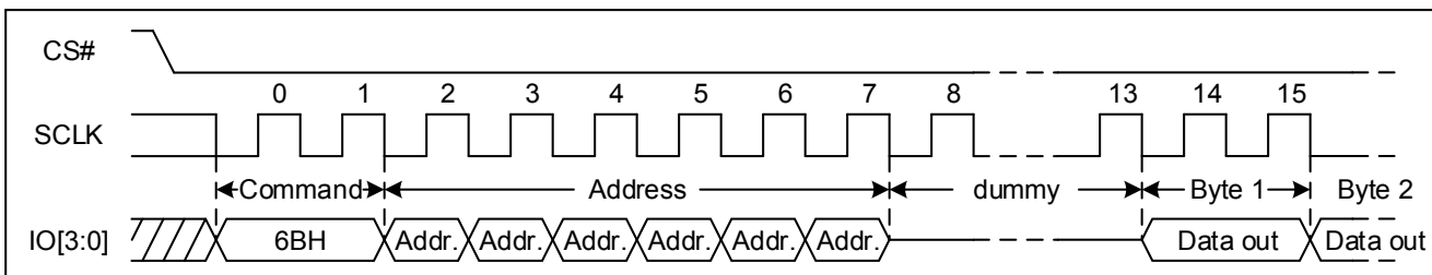
Figure 33 Quad Output Fast Read Sequence Diagram (QPI)
