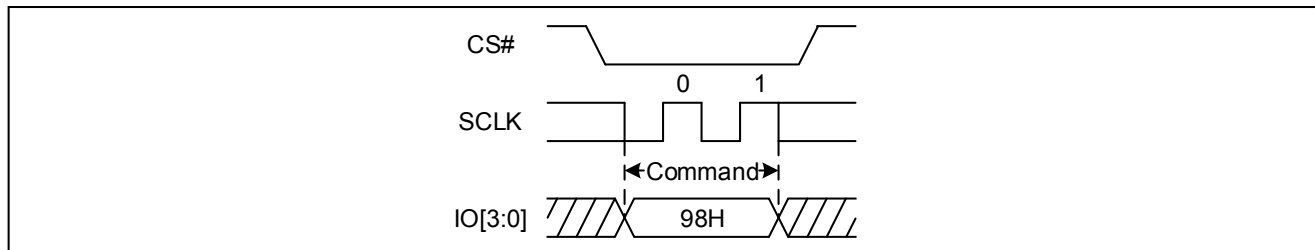
Figure 83 Global Block/Sector Unlock Sequence Diagram (QPI)
