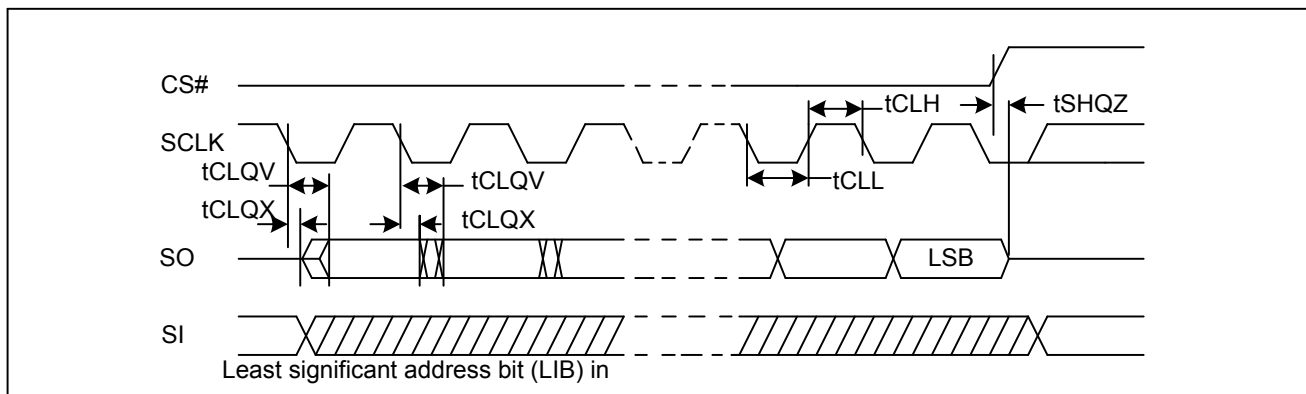
Figure 92. Output Timing
