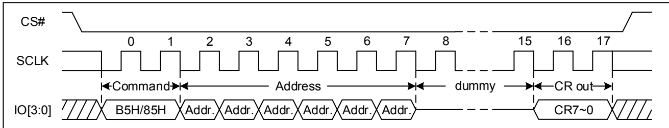
Figure 26 Read Configuration Registers Sequence (QPI)
