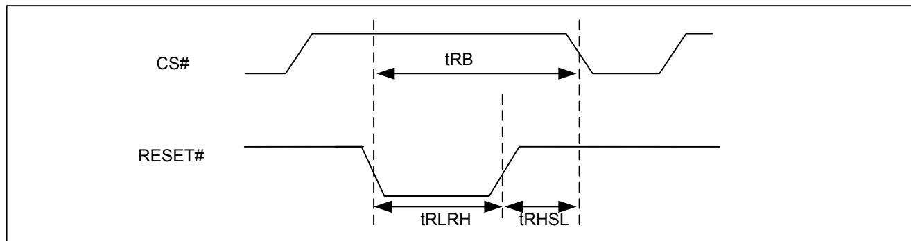
Figure 97. RESET Timing
