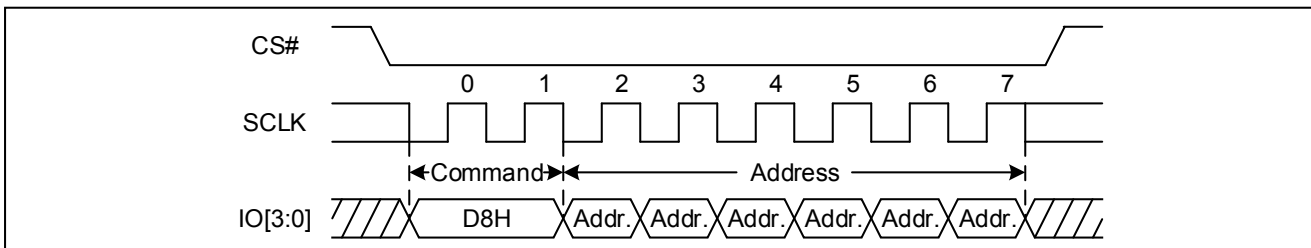
Figure 51 64KB Block Erase Sequence Diagram (QPI)
