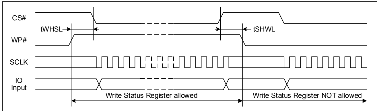
Figure 96. WP# Timing
