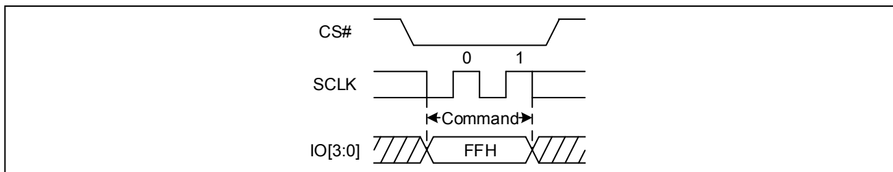
Figure 55 Disable QPI mode command Sequence Diagram
