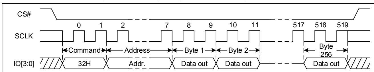
Figure 43 Quad Page Program Sequence Diagram (QPI)
