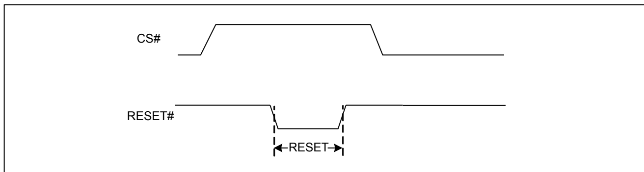
Figure 2 RESET Condition
