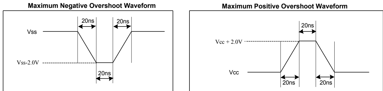
Figure 89. Input Test Waveform and Measurement Level
