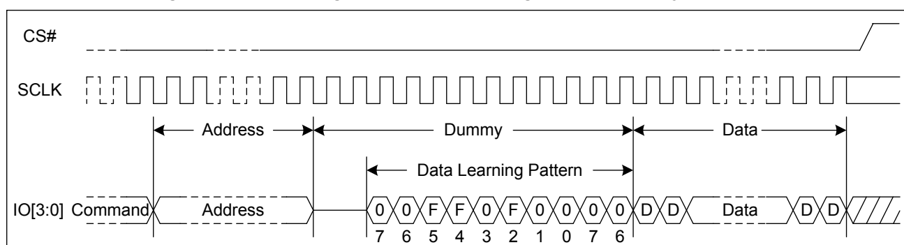
Figure 3. Data Learning Pattern Sequence Diagram (STR, Dummy Clock \geq 10 )
