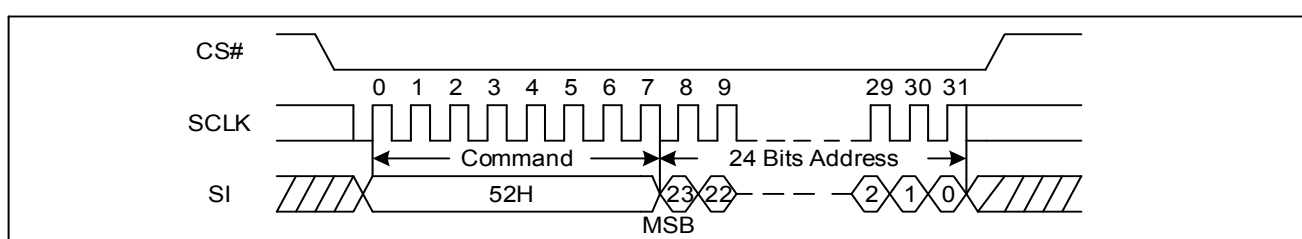
Figure 48 32KB Block Erase Sequence Diagram (SPI)
