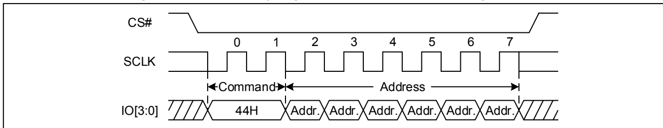
Figure 69 Erase Security Registers command Sequence Diagram (QPI)
