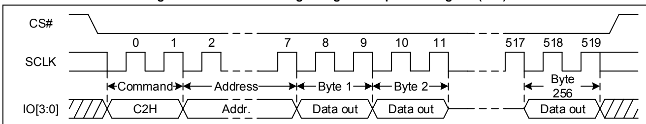
Figure 45 Extend Quad Page Program Sequence Diagram (QPI)
