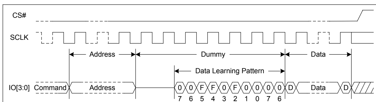
Figure 5. Data Learning Pattern Sequence Diagram (DTR, Dummy Clock \geq 6 )
