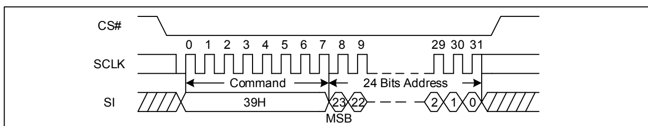
Figure 76 Individual Block/Sector Unlock command Sequence Diagram (SPI)
