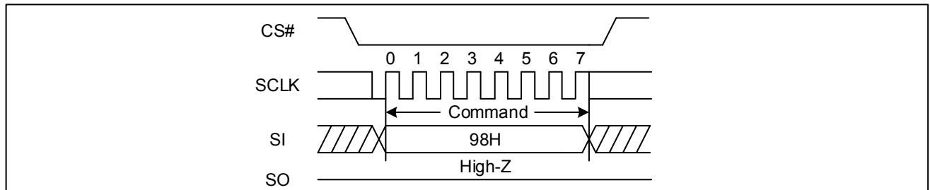
Figure 82 Global Block/Sector Unlock Sequence Diagram (SPI)
