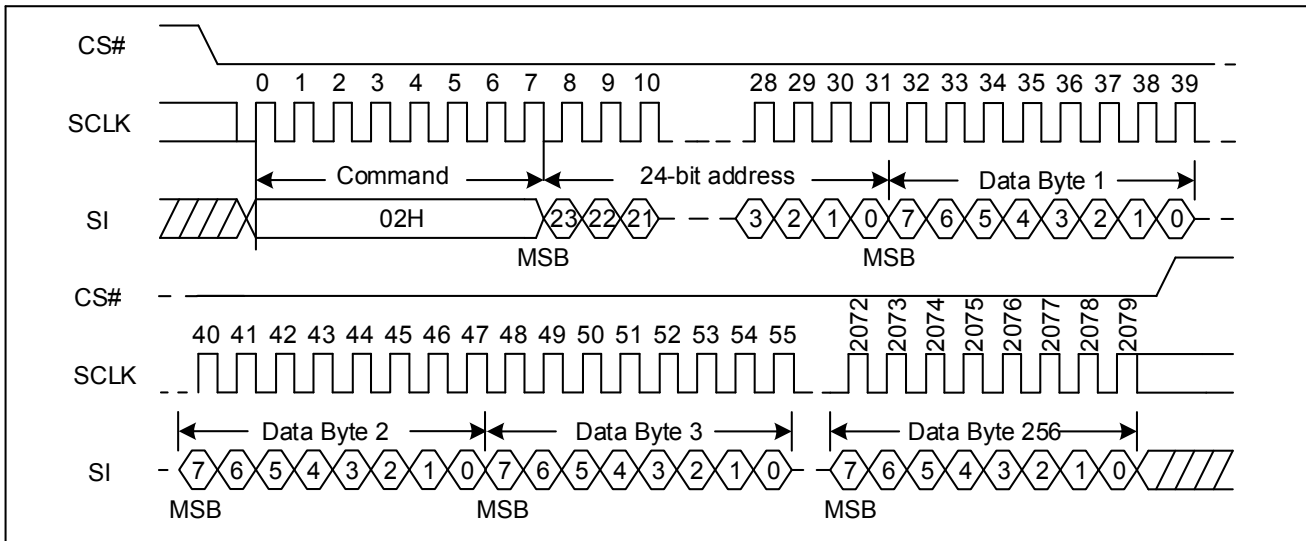
Figure 40 Page Program Sequence Diagram (SPI)
