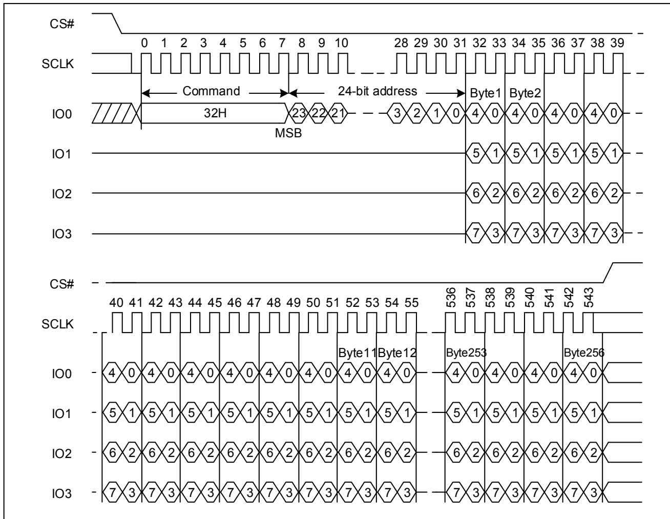
Figure 42 Quad Page Program Sequence Diagram (SPI)
