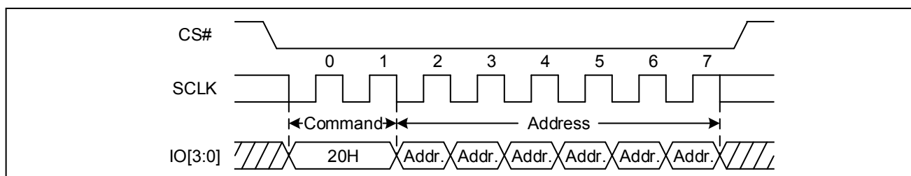
Figure 47 Sector Erase Sequence Diagram (QPI)
