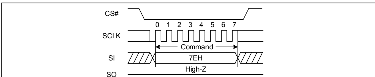
Figure 80 Global Block/Sector Lock Sequence Diagram (SPI)
