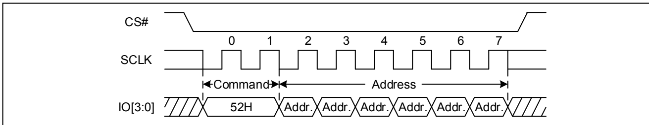
Figure 49 32KB Block Erase Sequence Diagram (QPI)
