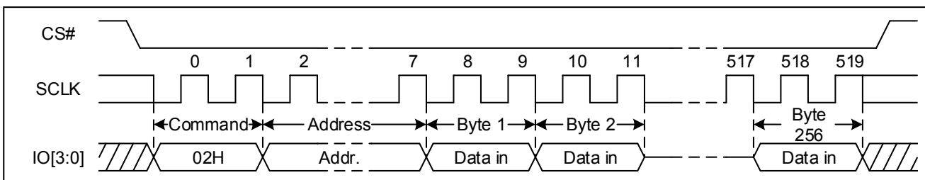
Figure 41 Page Program Sequence Diagram (QPI)
