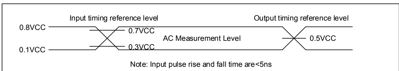
Figure 90. Absolute Maximum Ratings Diagram
