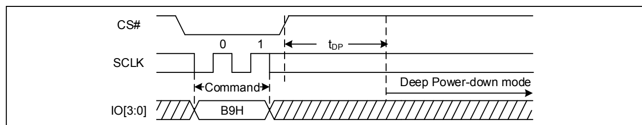
Figure 57 Deep Power-Down Sequence Diagram (QPI)
