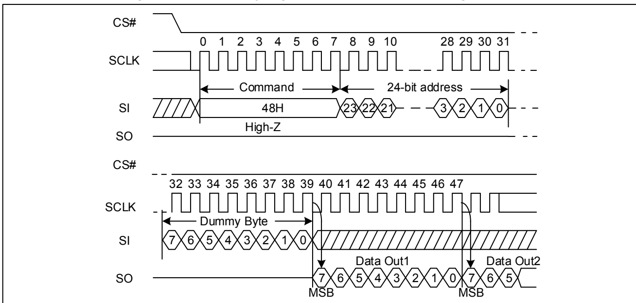
Figure 72 Read Security Registers command Sequence Diagram (SPI)
