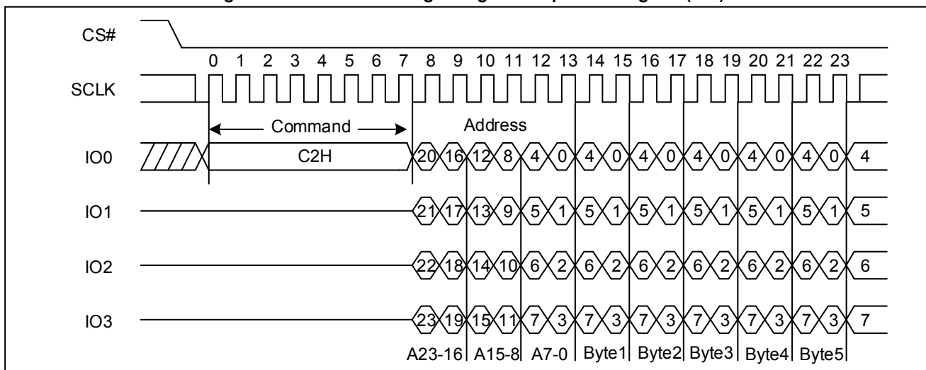
Figure 44 Extend Quad Page Program Sequence Diagram (SPI)
