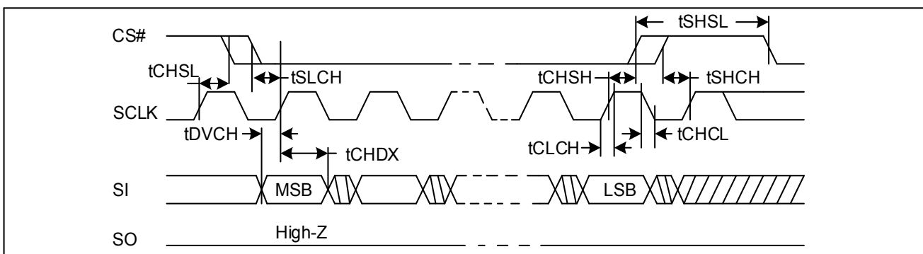
Figure 91. Serial Input Timing
