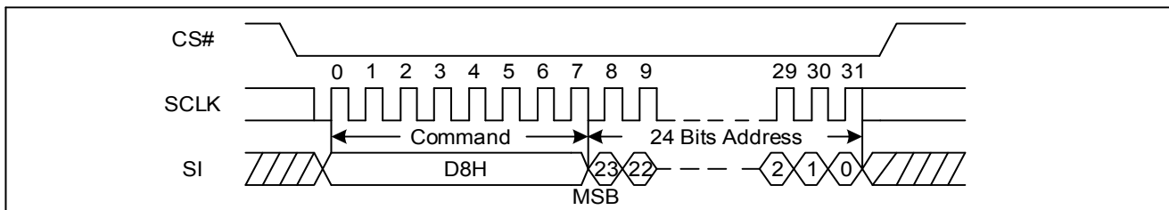
Figure 50 64KB Block Erase Sequence Diagram (SPI)
