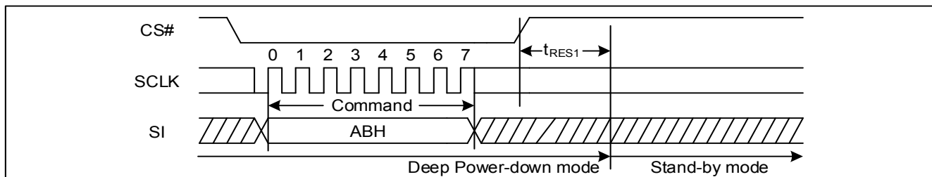
Figure 58 Release Power-Down Sequence Diagram (SPI)
