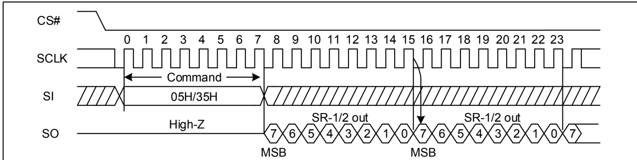
Figure 23 Read Status Register Sequence Diagram (SPI)
