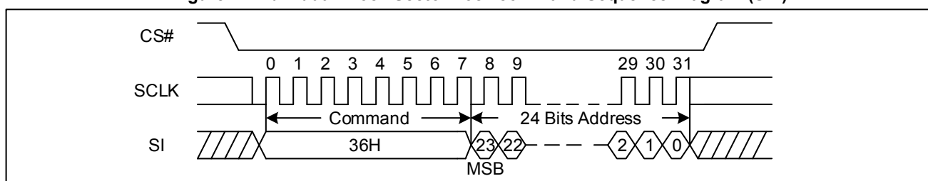
Figure 74 Individual Block/Sector Lock command Sequence Diagram (SPI)
