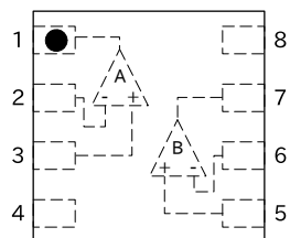
WSON8-2×2(TOP VIEW)
