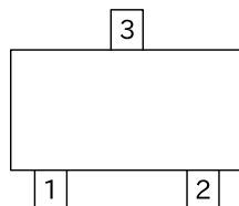
SOT-23(TOP VIEW)
