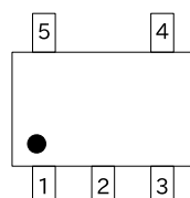
SC-70-5(TOP VIEW)
