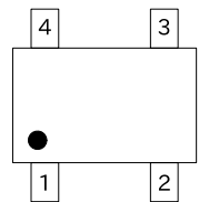
SC-82AB(TOP VIEW)
