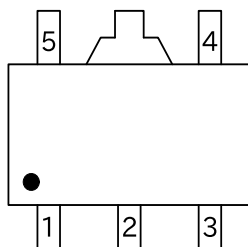
SOT-89-5(TOP VIEW)
