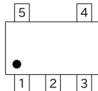
SOT-25(TOP VIEW)
