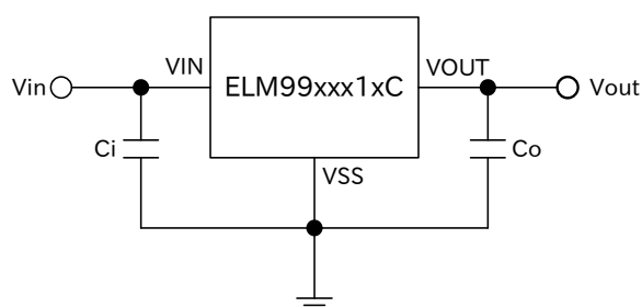
ELM99xxx1xC
