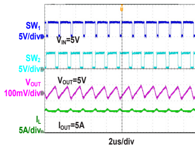
Steady State Test (Buck-Boost)
