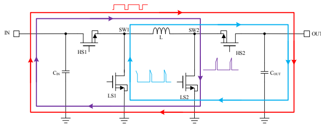
Buck-Boost Mode
