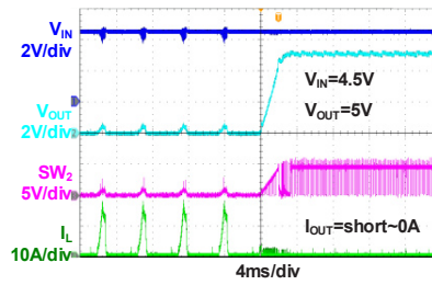
Short Protection (Boost)
