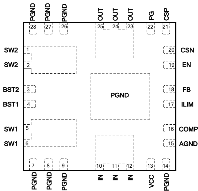
QFN28-5×5(TOP VIEW)
