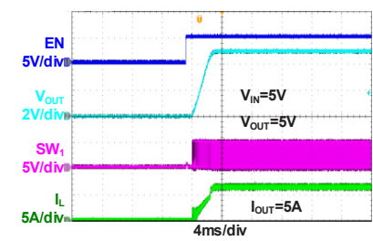
EN Power on (Buck-Boost)
