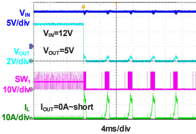
Short Protection (Buck)
