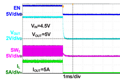
EN Power off (Boost)
