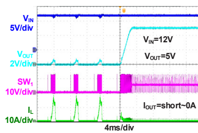
Short Protection (Buck)
