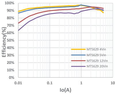
Steady State Test (Boost)
