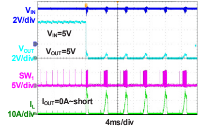
Short Protection (Buck-Boost)
