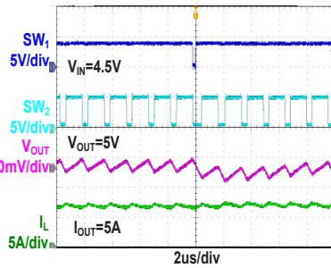
Steady State Test (Boost)
