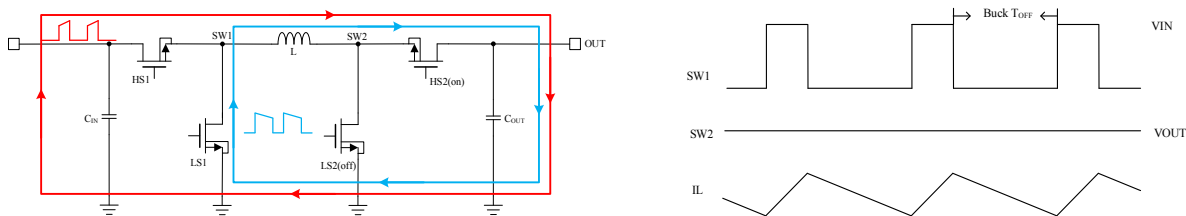
Buck Mode
