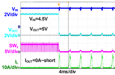
Short Protection (Boost)
