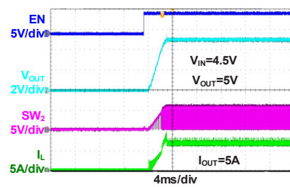
EN Power on (Boost)
