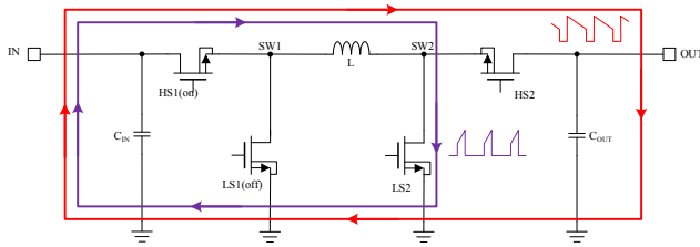
Boost Mode
