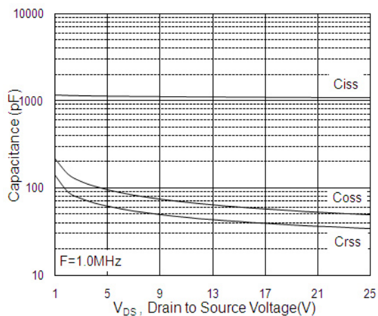
Fig.7 Capacitance
