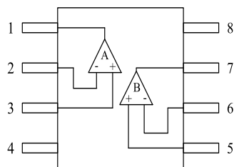
SOP-8(俯视图)
