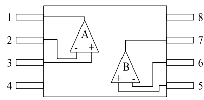
TSSOP-8(俯视图)
