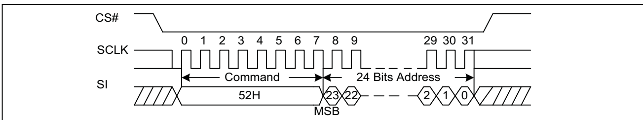
Figure18. 32KB Block Erase Sequence Diagram (SPI)
