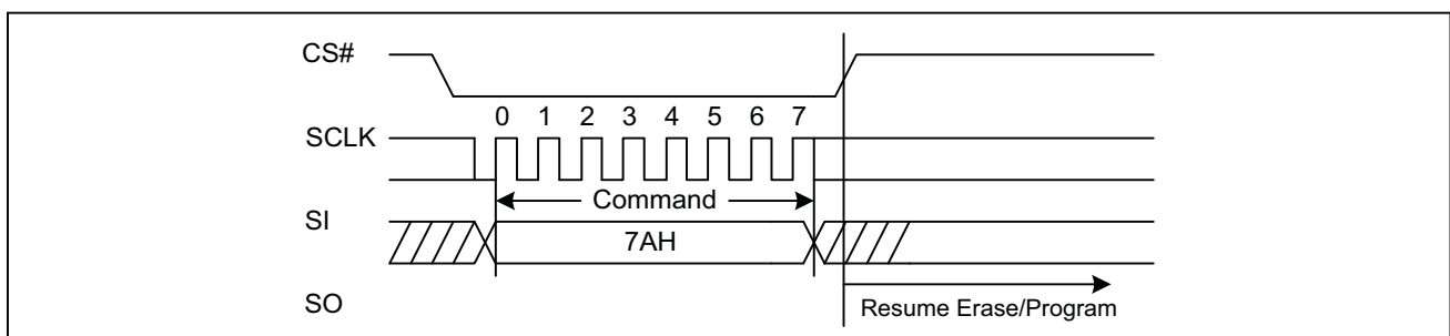
Figure29. Program/Erase Resume Sequence Diagram (SPI)
