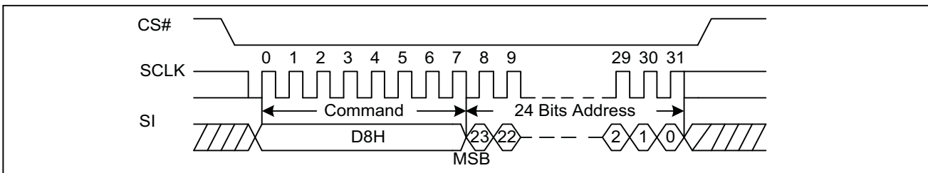
Figure19. 64KB Block Erase Sequence Diagram
