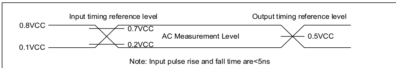
Figure 42. Input/Output Timing Reference Level
