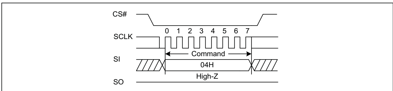
Figure3. Write Disable Sequence Diagram (SPI)
