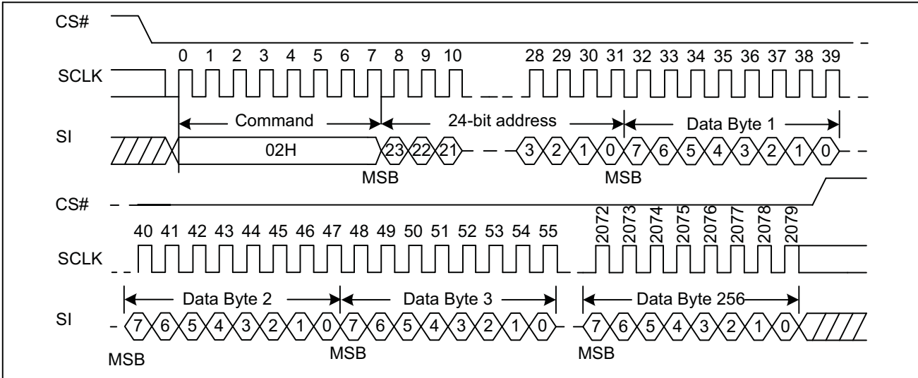
Figure15. Page Program Sequence Diagram (SPI)
