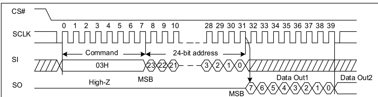
Figure7. Read Data Bytes Sequence Diagram (SPI)
