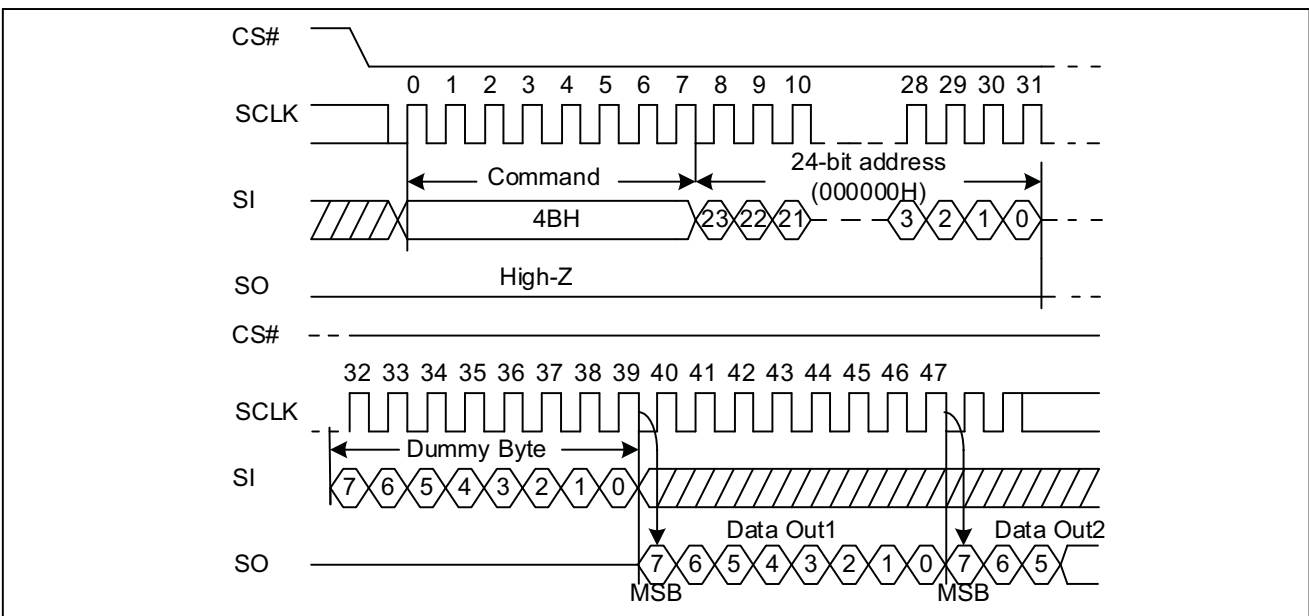
Figure30. Read Unique ID Sequence Diagram (SPI)
