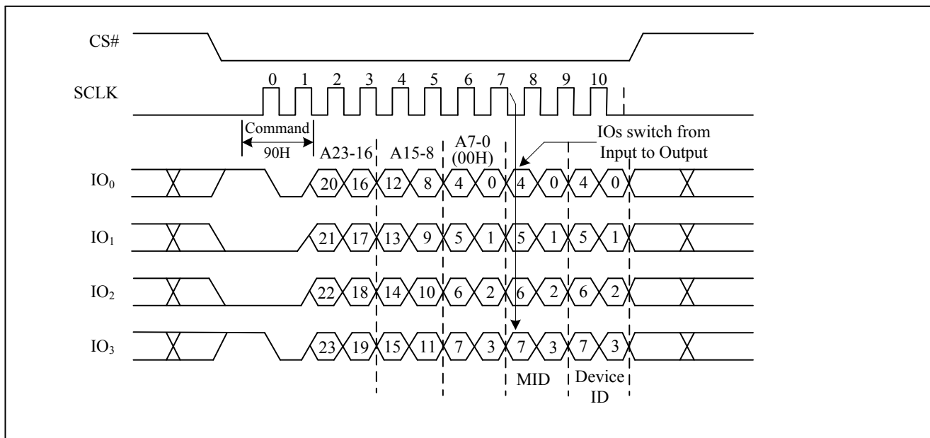
Figure26a. Read Manufacturer ID/ Device ID Sequence Diagram (QPI)
