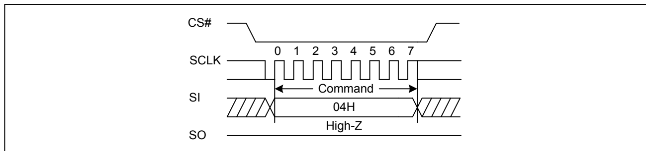
Figure5. Write Disable Sequence Diagram
