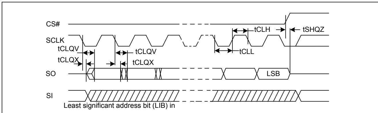
Figure48. Output Timing
