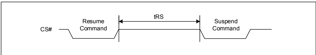
Figure45. Resume to Suspend Timing
