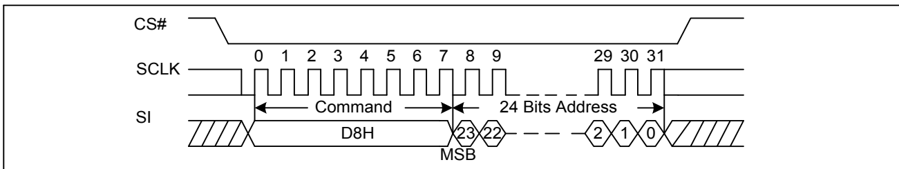
Figure 20. 64KB Block Erase Sequence Diagram
