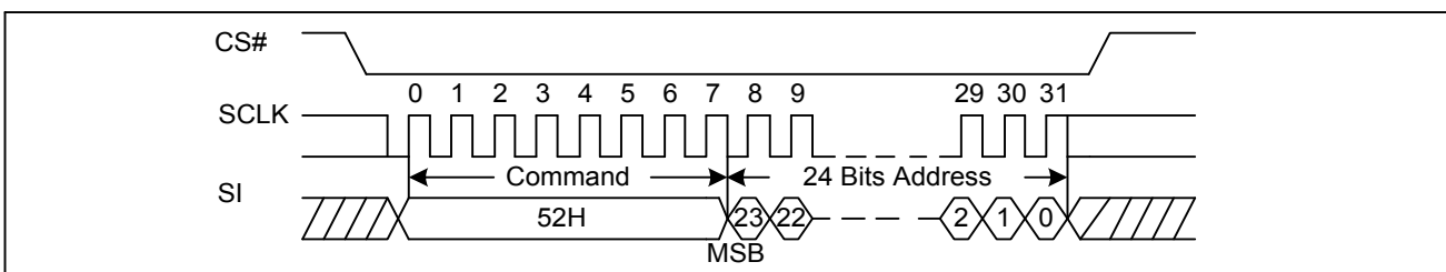
Figure 19. 32KB Block Erase Sequence Diagram
