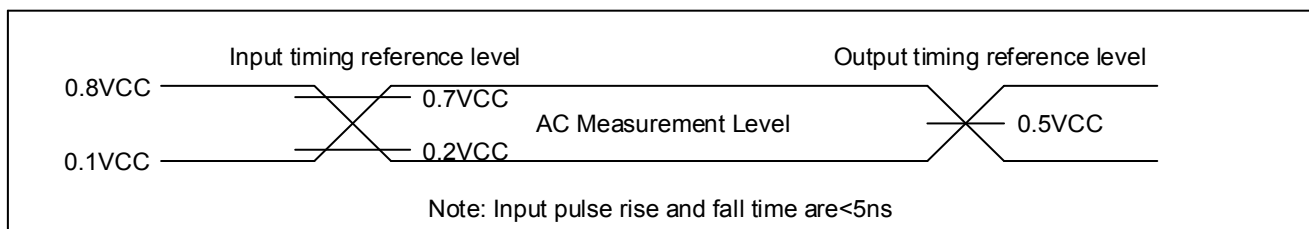
Figure 40. Input Test Waveform and Measurement Level
