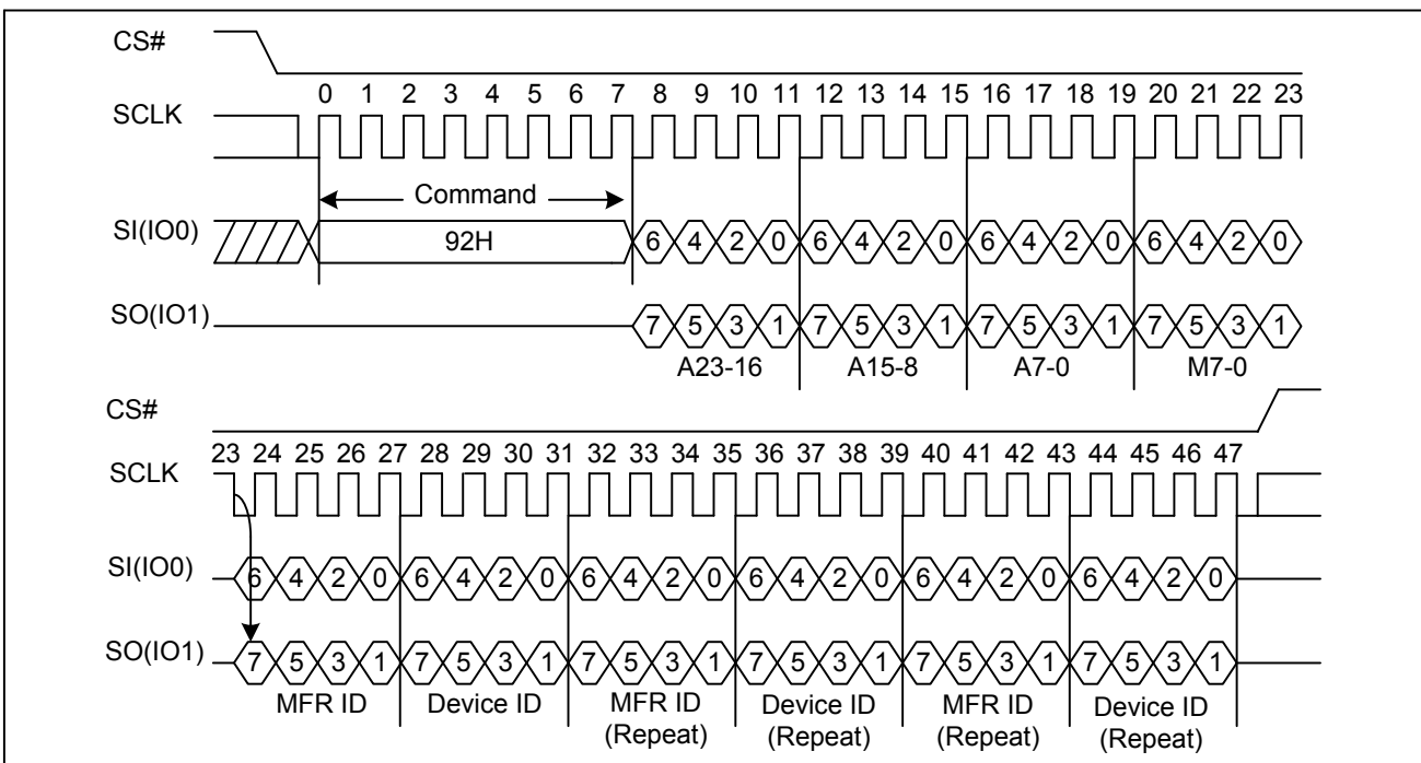
Figure 27. Read Manufacture ID/ Device ID Dual I/O Sequence Diagram
