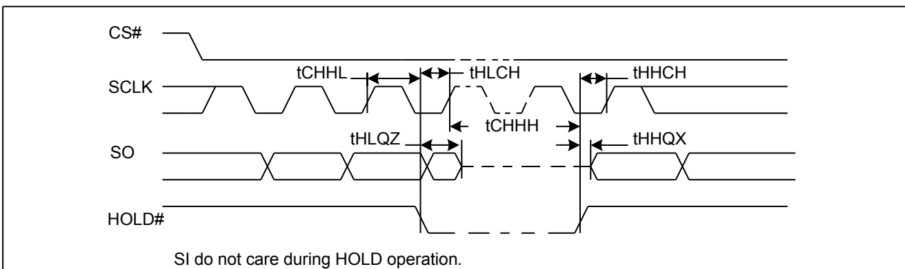
Figure 44. Hold Timing
