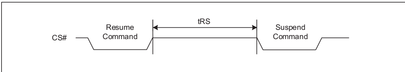
Figure46. Resume to Suspend Timing Diagram
