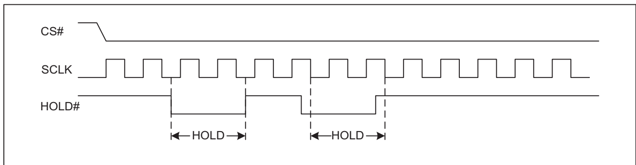
Figure1. Hold Condition
