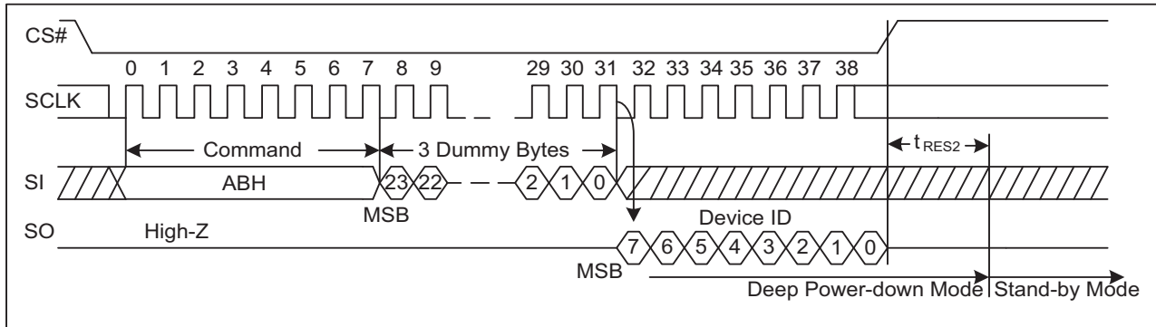
Figure23. Release Power-Down/Read Device ID Sequence Diagram
