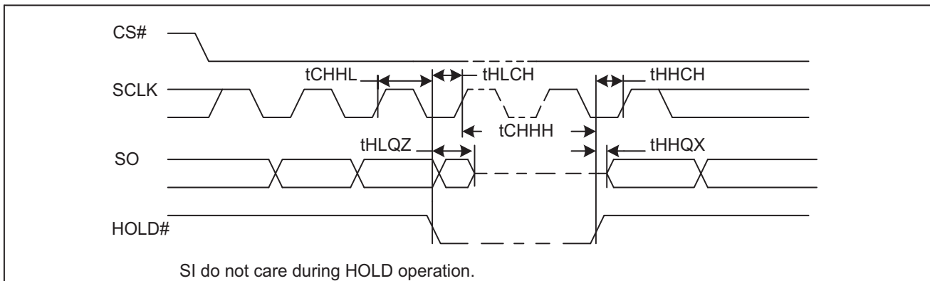
Figure47. Hold Timing
