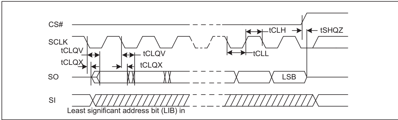
Figure45. Output Timing
