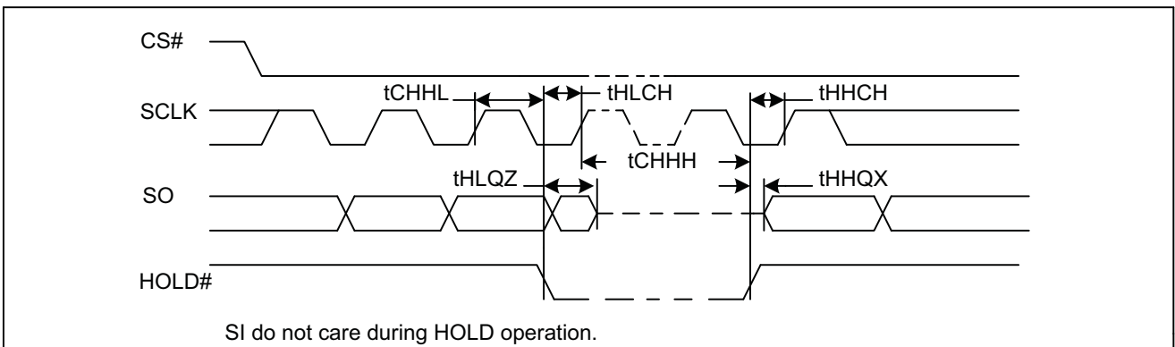
Figure46. Hold Timing
