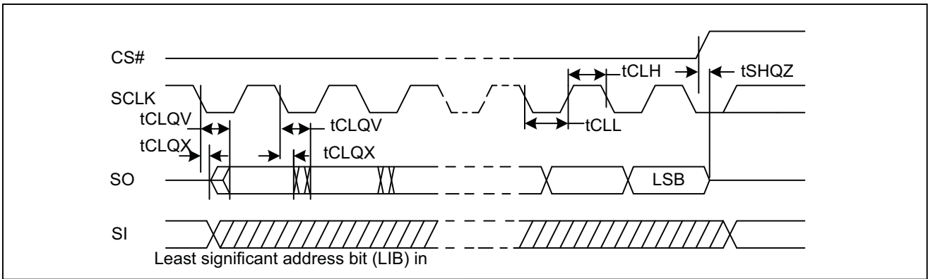
Figure44. Output Timing
