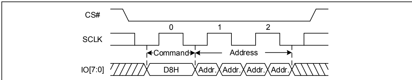
Figure 70. 64KB Block Sequence Diagram (DTR OPI)
