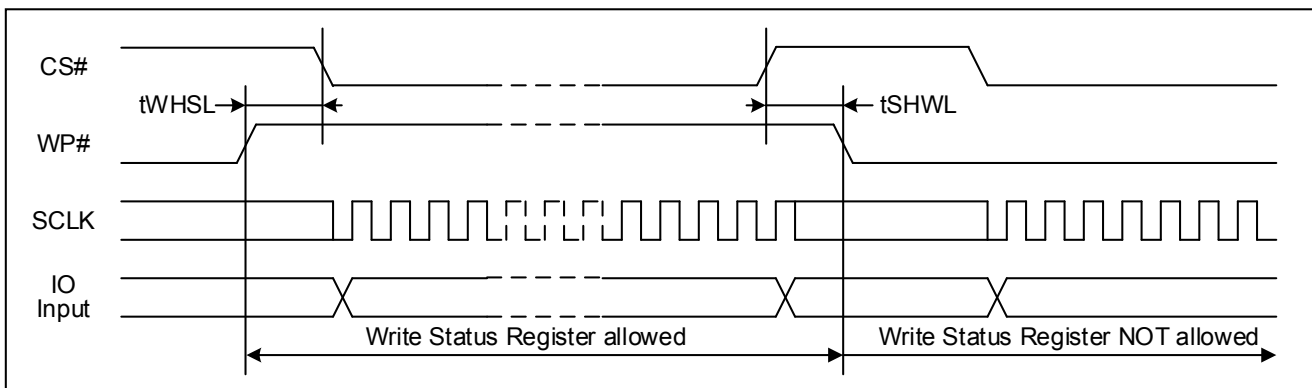
Figure 124. WP# Timing
