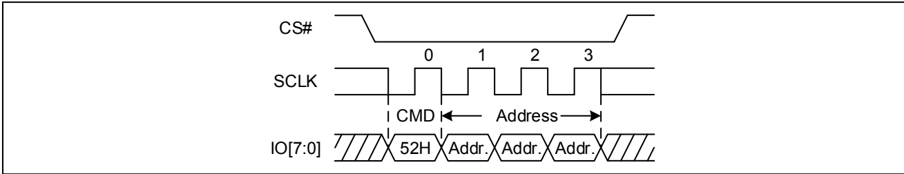
Figure 66. 32KB Block Erase Sequence Diagram (STR OPI)
