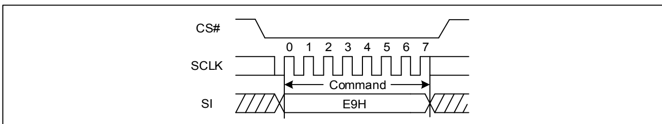
Figure 12. Disable 4-Byte Mode Sequence Diagram (SPI)
