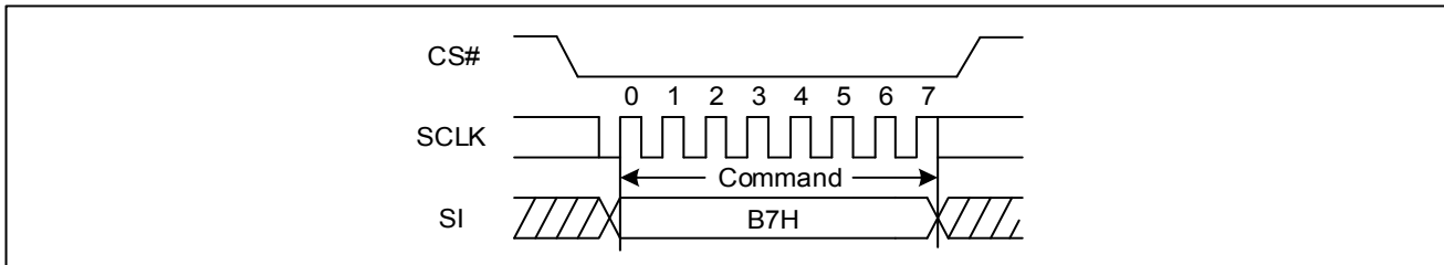
Figure 10. Enable 4-Byte Mode Sequence Diagram (SPI)
