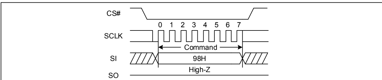
Figure 107. The Global Block/Sector Unlock Sequence Diagram (SPI)
