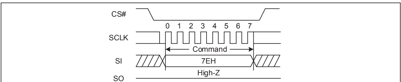
Figure 105. The Global Block/Sector Lock Sequence Diagram (SPI)
