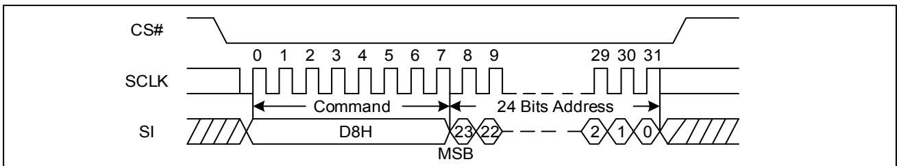
Figure 68. 64KB Block Erase Sequence Diagram (SPI)
