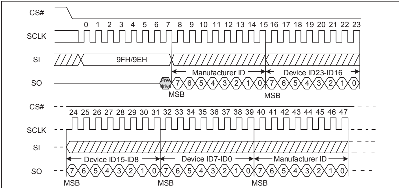
Figure 80. Read Identification ID Sequence Diagram (SPI)
