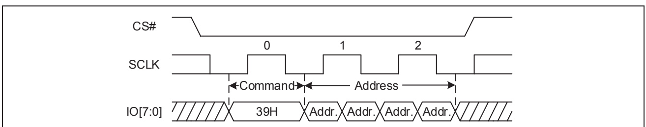
Figure 101. Individual Block/Sector Unlock command Sequence Diagram (DTR OPI)
