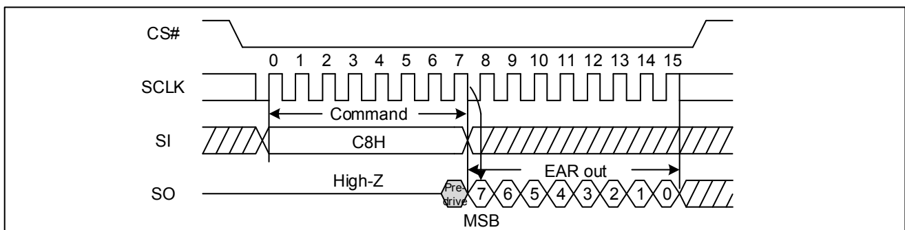
Figure 36. Read Extended Address Register Sequence Diagram (SPI)
