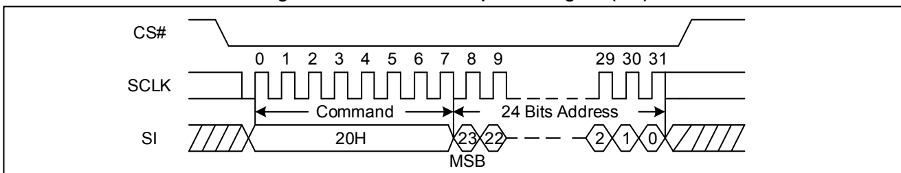
Figure 62. Sector Erase Sequence Diagram (SPI)
