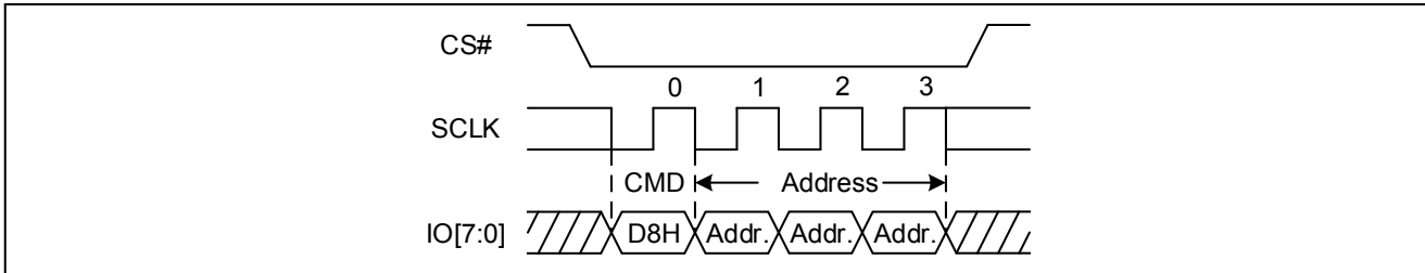
Figure 69. 64KB Block Sequence Diagram (STR OPI)
