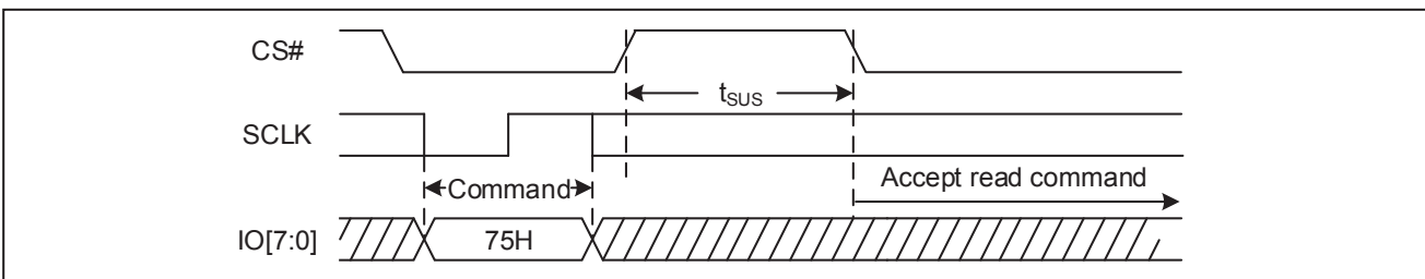
Figure 84. Program/Erase Suspend Sequence Diagram (OPI)
