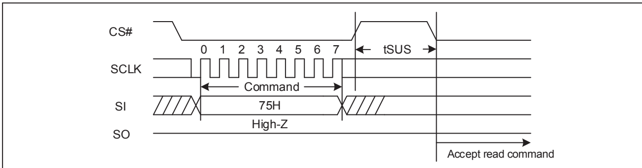
Figure 83. Program/Erase Suspend Sequence Diagram (SPI)
