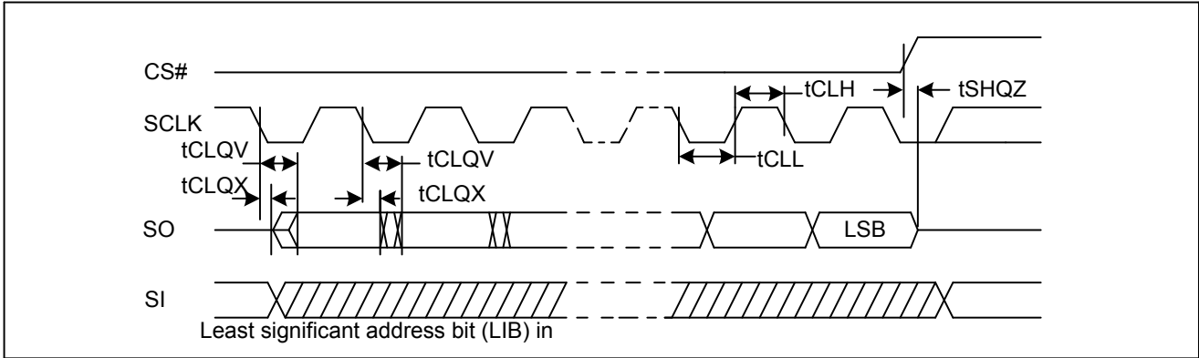
Figure 118. Output Timing
