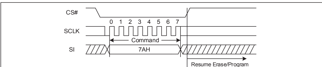
Figure 85. Program/Erase Resume Sequence Diagram (SPI)
