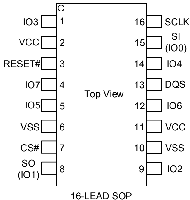
Figure 1 Connection Diagram for SOP16 package
