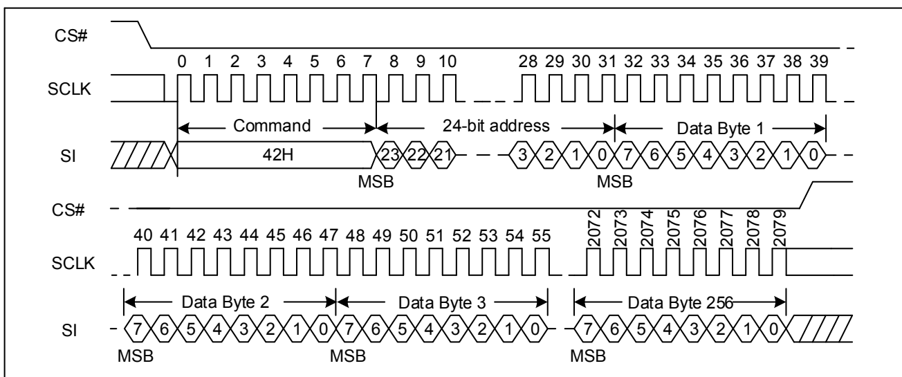
Figure 90. Program Security Registers command Sequence Diagram (SPI)
