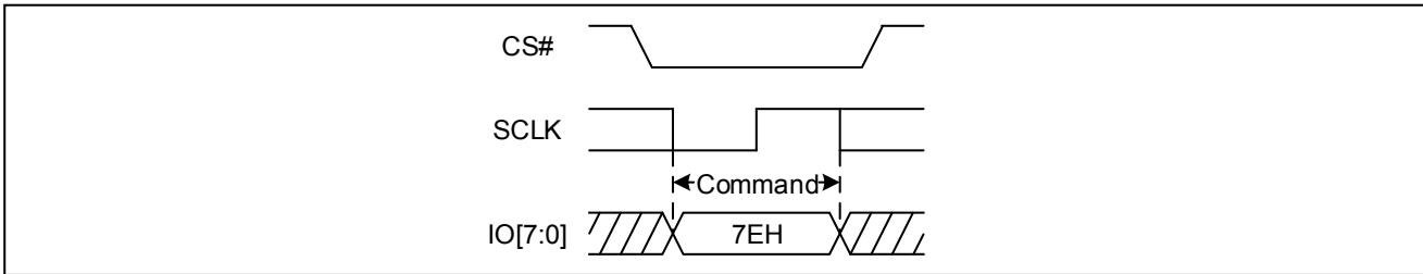
Figure 106. The Global Block/Sector Lock Sequence Diagram (OPI)
