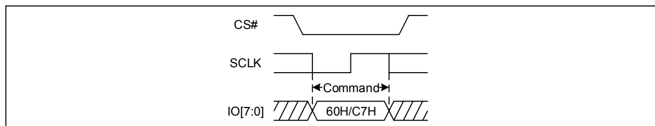
Figure 72. Chip Erase Sequence Diagram (OPI)
