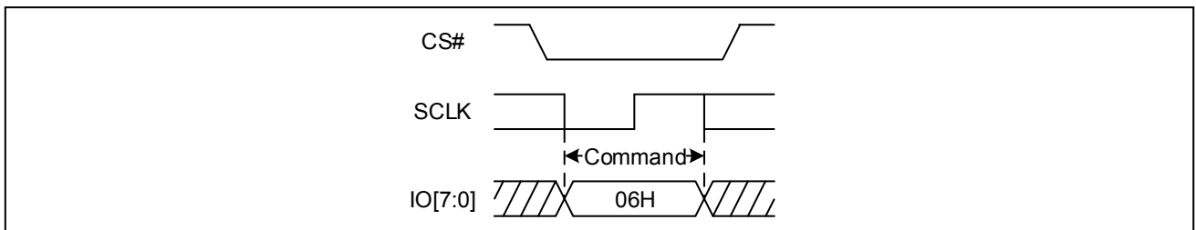
Figure 15. Write Enable Sequence Diagram (OPI)
