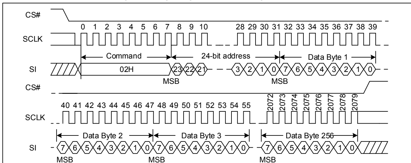
Figure 53. Page Program Sequence Diagram (SPI)
