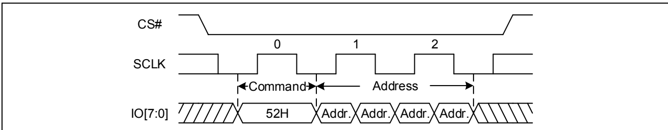
Figure 67. 32KB Block Erase Sequence Diagram (DTR OPI)
