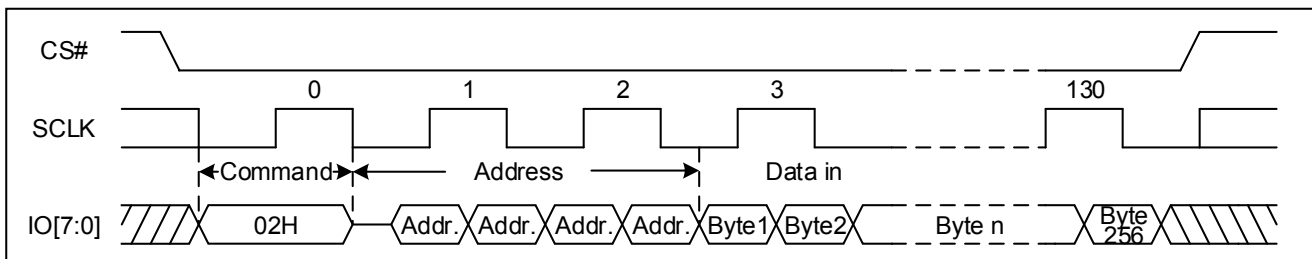
Figure 55. Page Program Sequence Diagram (DTR OPI)
