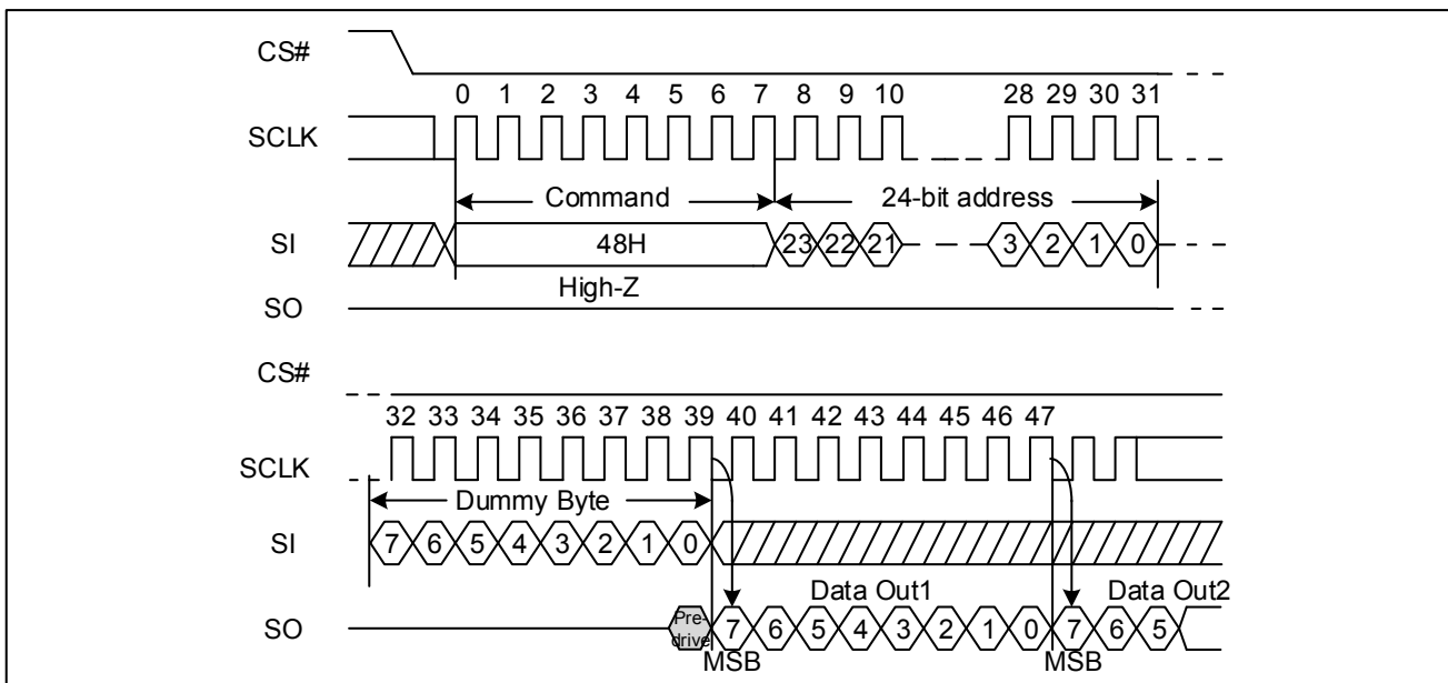
Figure 93. Read Security Registers command Sequence Diagram (SPI)
