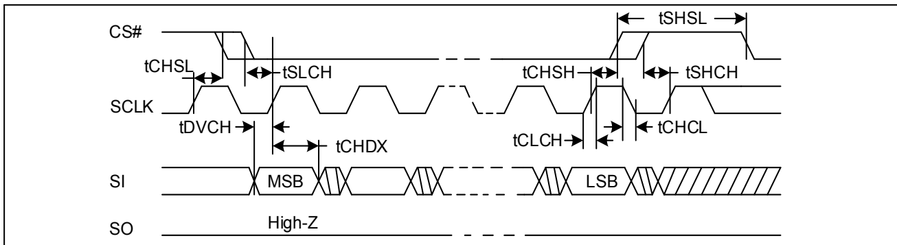
Figure 117. Serial Input Timing
