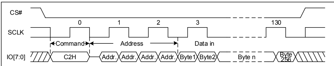
Figure 61. Page Program Sequence Diagram (DTR OPI)
