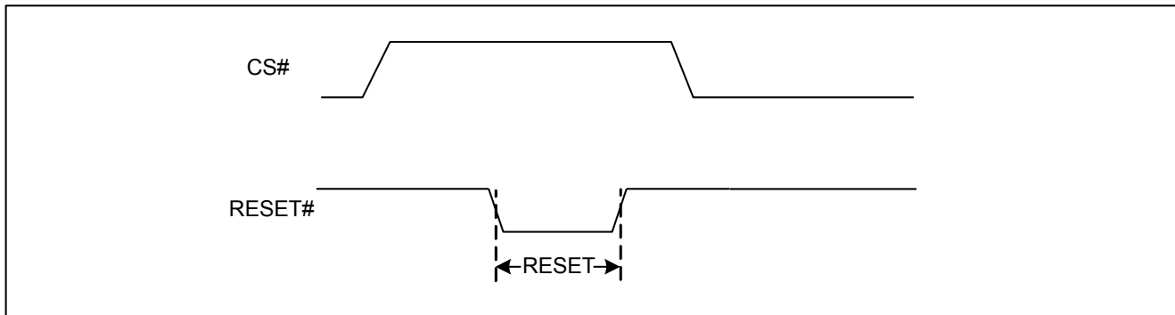
Figure 3 RESET Condition
