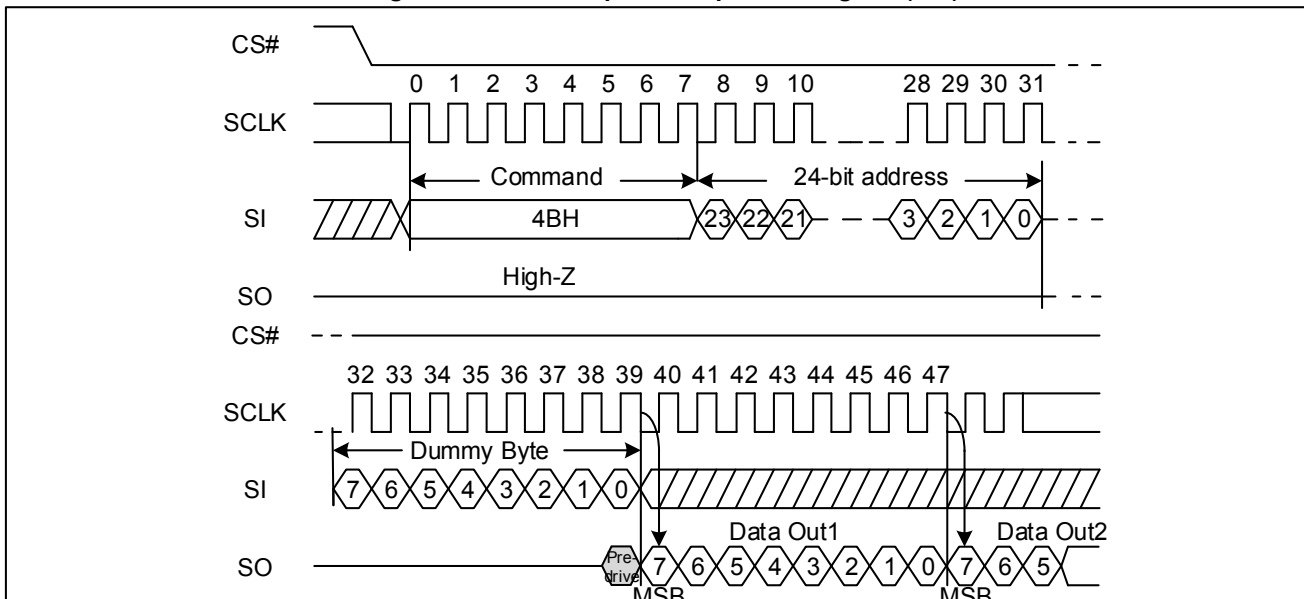
Figure 77. Read Unique ID Sequence Diagram (SPI)
