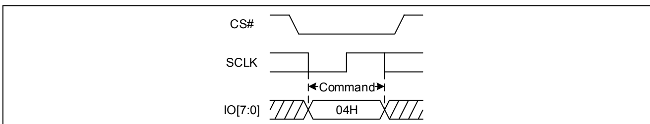
Figure 17. Write Disable Sequence Diagram (OPI)
