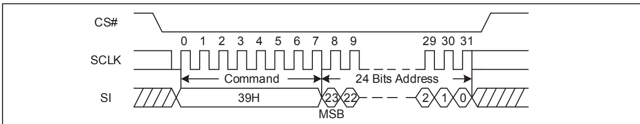
Figure 99. Individual Block/Sector Unlock command Sequence Diagram (SPI)
