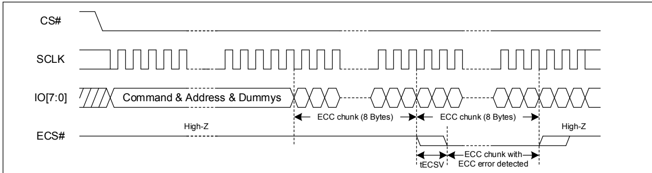
Figure 4. ECS# Timing
