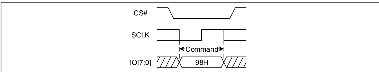
Figure 108. The Global Block/Sector Unlock Sequence Diagram (OPI)
