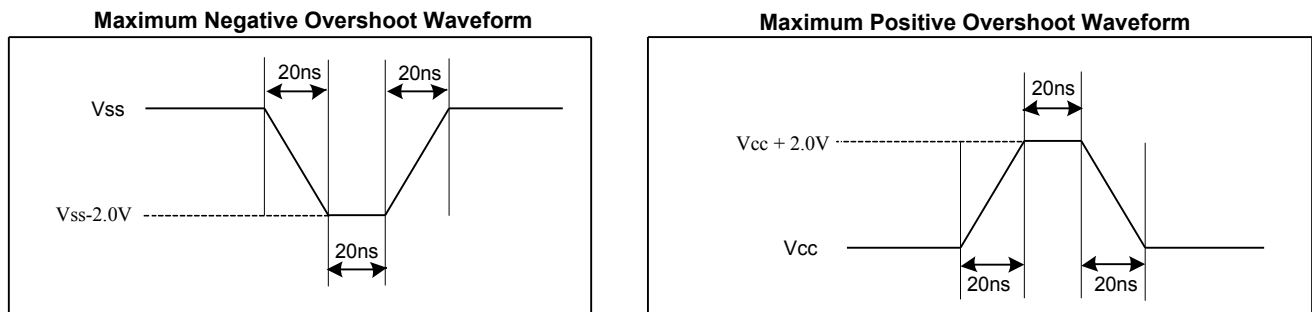
Figure 115. Input Test Waveform and Measurement Level
