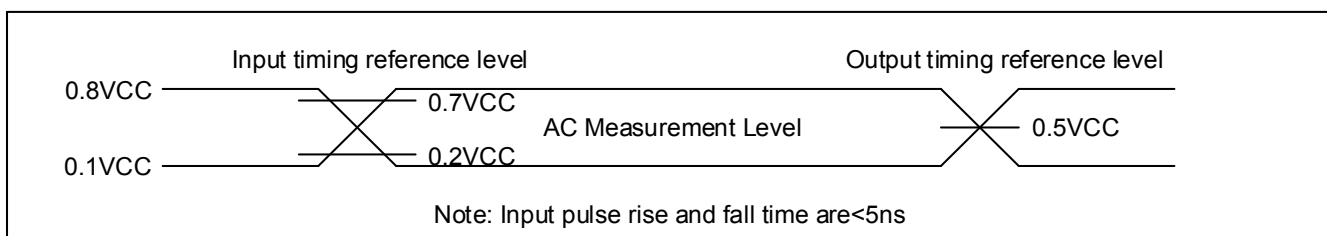
Figure 116. Absolute Maximum Ratings Diagram
