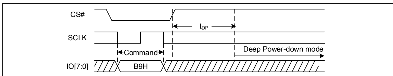
Figure 74. Deep Power-Down Sequence Diagram (OPI)
