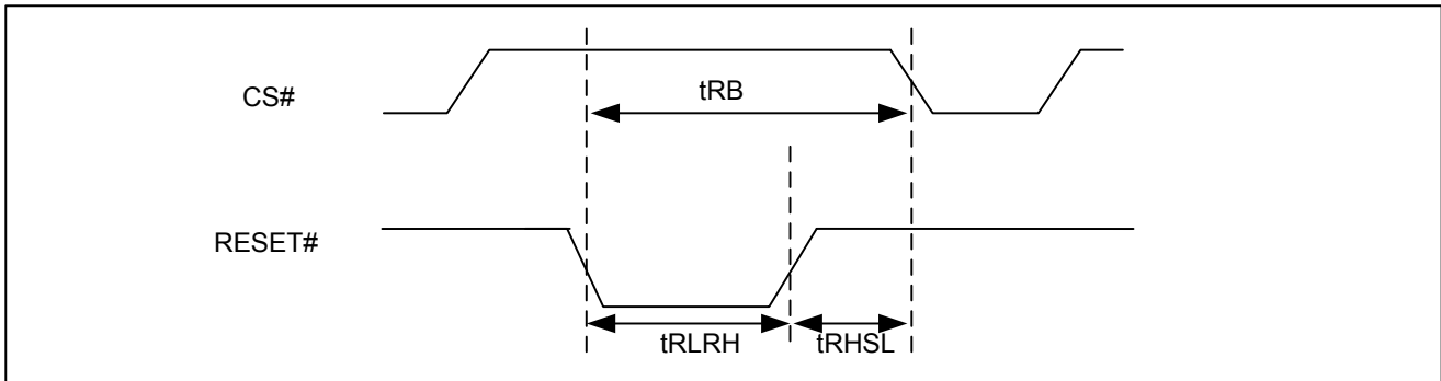
Figure 125. RESET Timing
