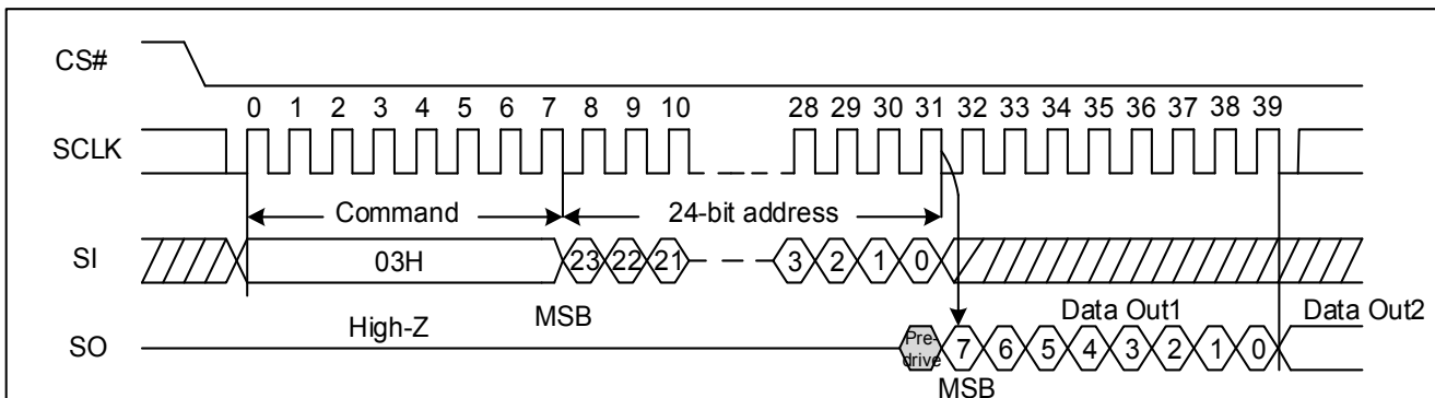
Figure 39. Read Data Bytes Sequence Diagram
