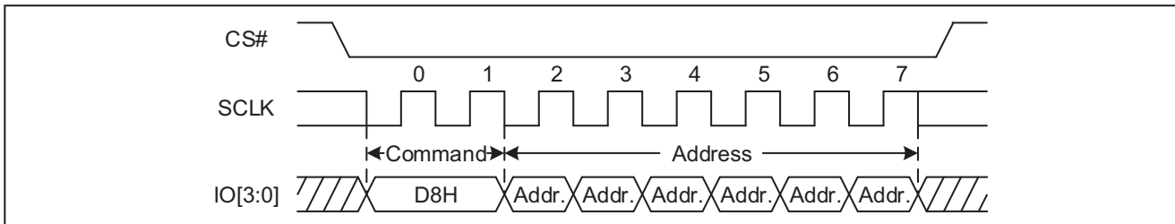
Figure 58 64KB Block Erase Sequence Diagram (QPI)
