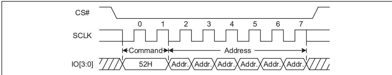
Figure 56 32KB Block Erase Sequence Diagram (QPI)
