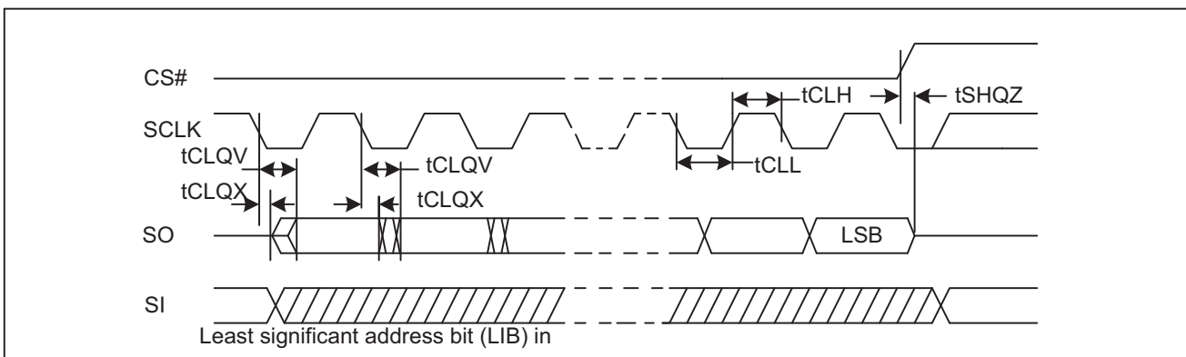
Figure 100. Output Timing
