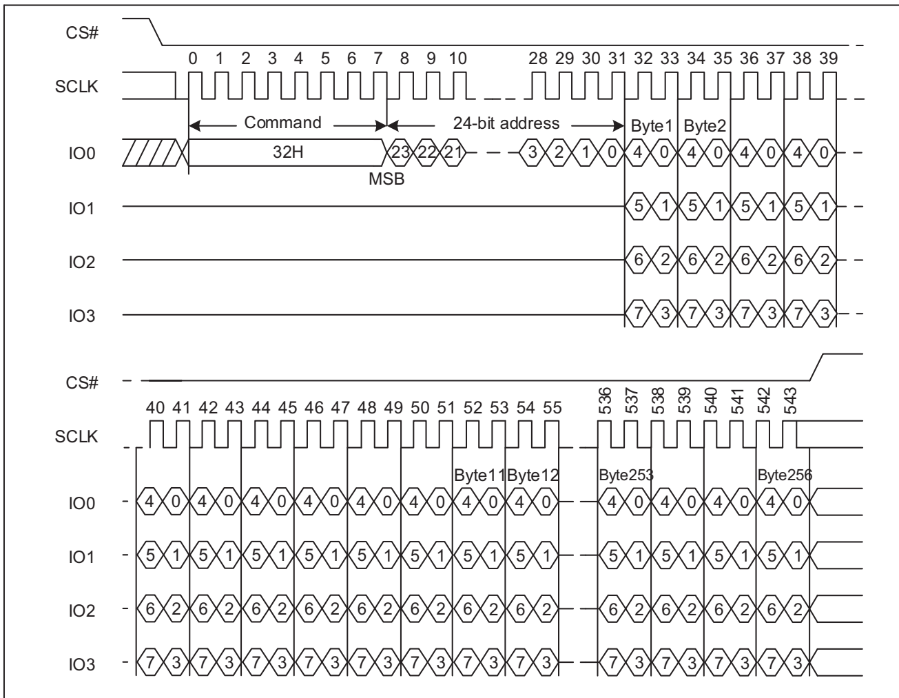
Figure 49 Quad Page Program Sequence Diagram (SPI)
