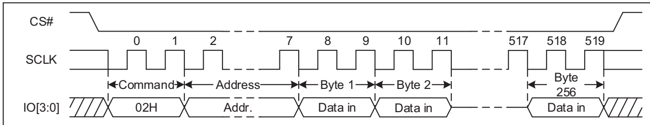
Figure 48 Page Program Sequence Diagram (QPI)
