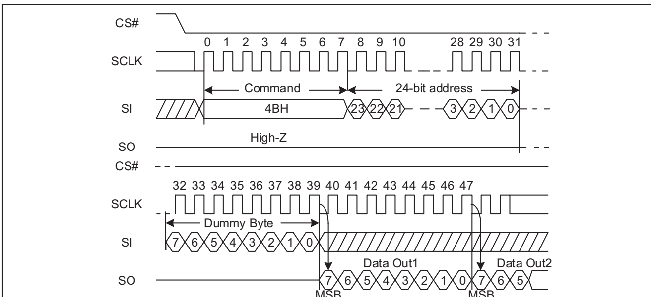
Figure 67 Read Unique ID Sequence Diagram (SPI)
