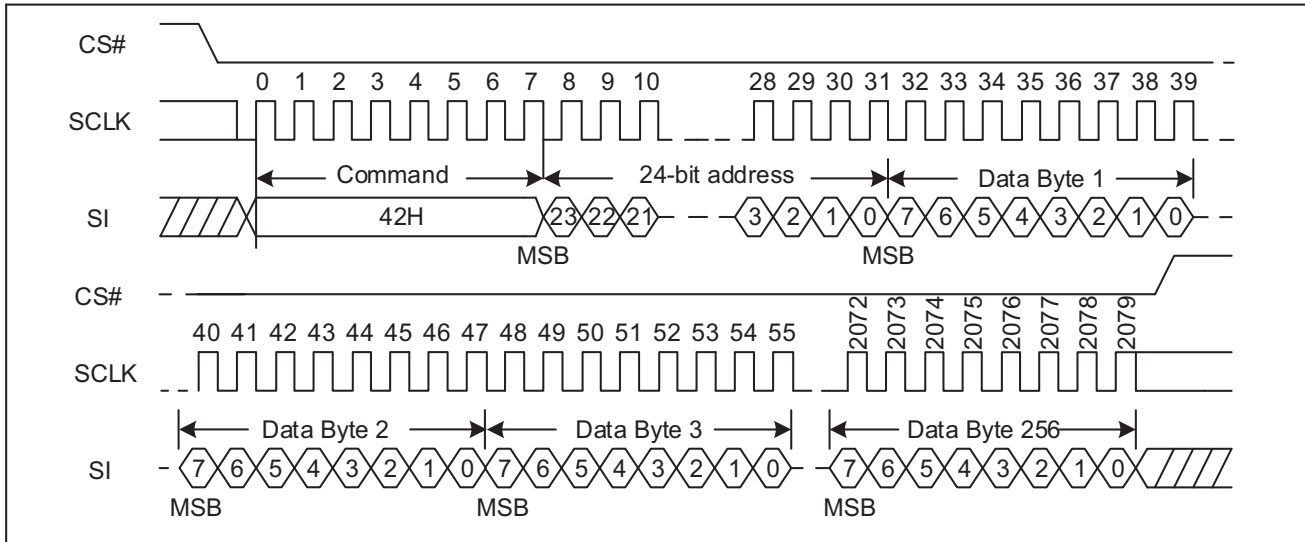
Figure 78 Program Security Registers command Sequence Diagram (SPI)
