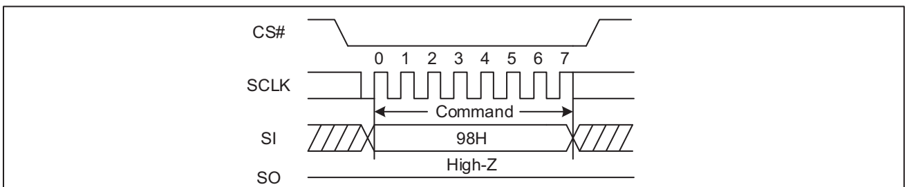
Figure 90 Global Block/Sector Unlock Sequence Diagram (SPI)
