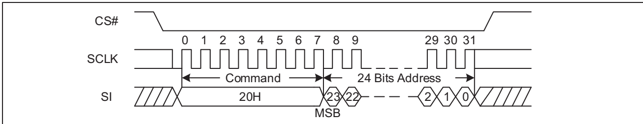
Figure 53 Sector Erase Sequence Diagram (SPI)
