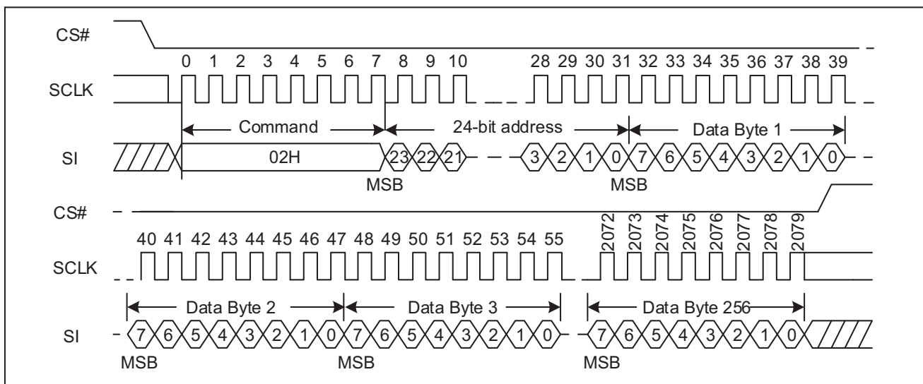
Figure 47 Page Program Sequence Diagram (SPI)
