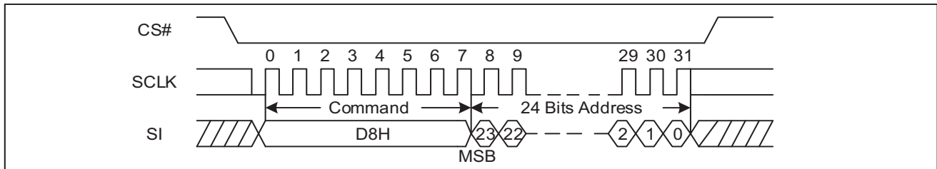
Figure 57 64KB Block Erase Sequence Diagram (SPI)
