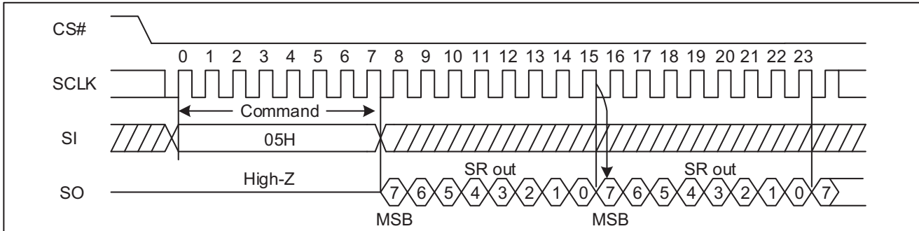
Figure 25 Read Status Register Sequence Diagram (SPI)
