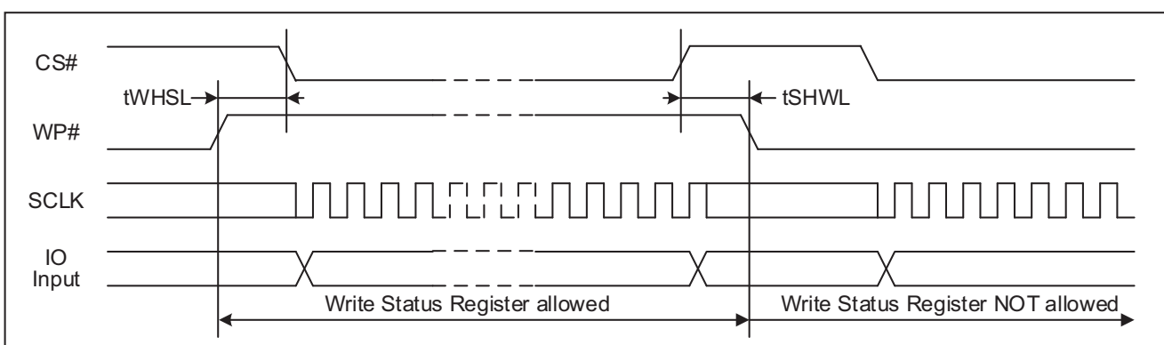
Figure 104. WP# Timing
