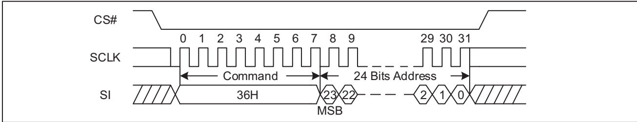
Figure 82 Individual Block/Sector Lock command Sequence Diagram (SPI)
