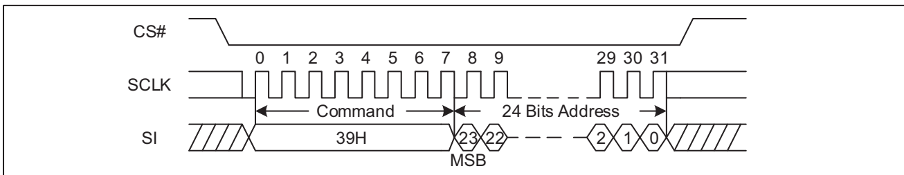
Figure 84 Individual Block/Sector Unlock command Sequence Diagram (SPI)
