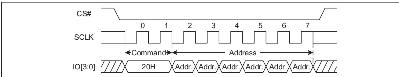
Figure 54 Sector Erase Sequence Diagram (QPI)
