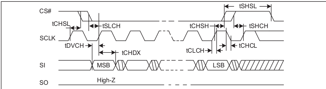
Figure 99. Serial Input Timing
