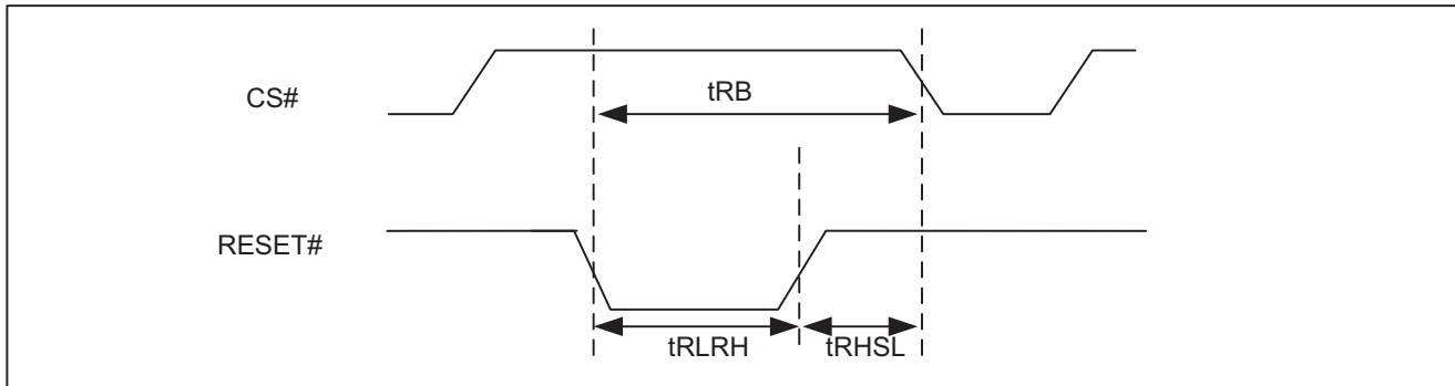
Figure 105. RESET Timing
