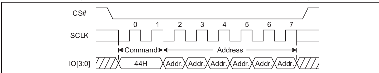
Figure 77 Erase Security Registers command Sequence Diagram (QPI)
