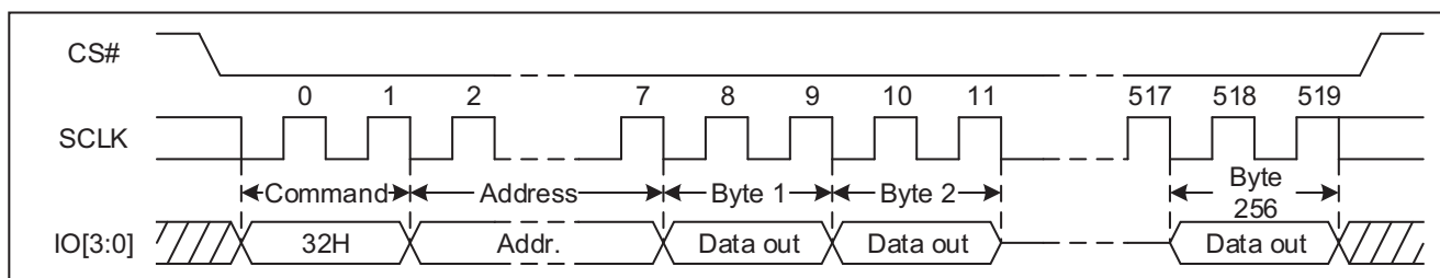
Figure 50 Quad Page Program Sequence Diagram (QPI)
