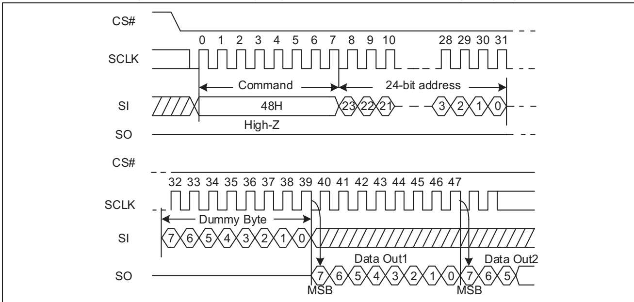
Figure 80 Read Security Registers command Sequence Diagram (SPI)
