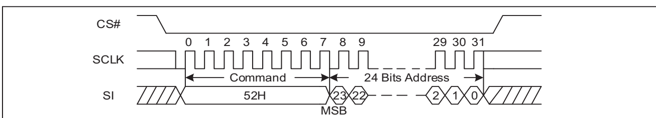
Figure 55 32KB Block Erase Sequence Diagram (SPI)
