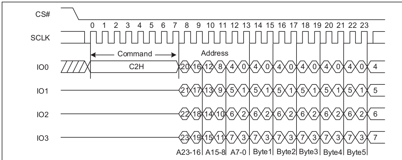
Figure 51 Extend Quad Page Program Sequence Diagram (SPI)
