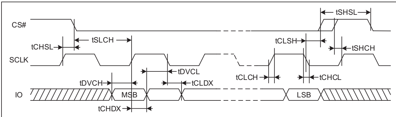
Figure 101. Serial Input Timing (DTR)
