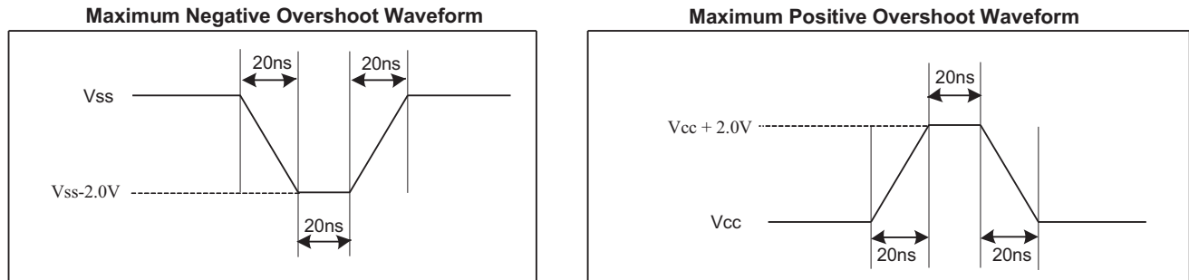
Figure 97. Input Test Waveform and Measurement Level
