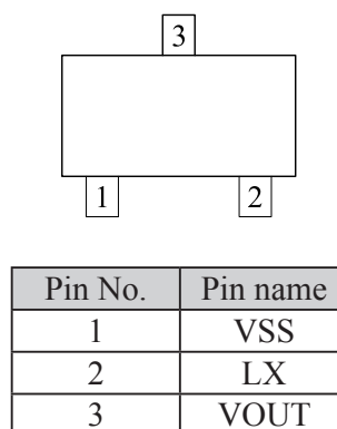
SOT-23(TOP VIEW)
