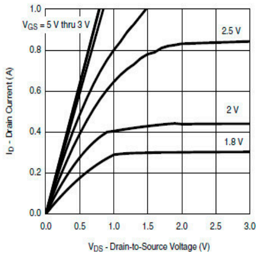
Output Characteristics
