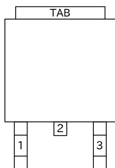
TO-252-3(TOP VIEW)
